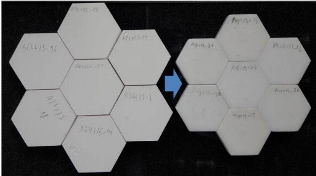
Figure 8. Several hexagonal alumina samples microwave sintered.
