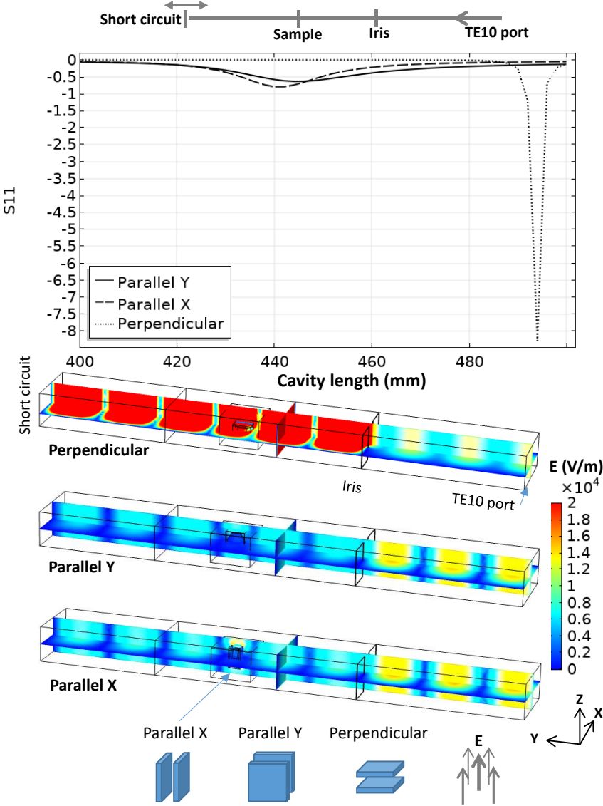
Figure 4. Resonant behavior of the 915 MHz cavity for three different orientations of the SiC susceptors plates with the E field; the simulation image corresponds to the minimum S_{11} parameter for each tested orientation.
