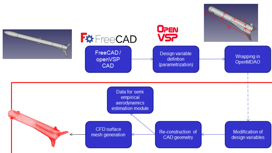
Figure 3: Illustration of geometry discipline
