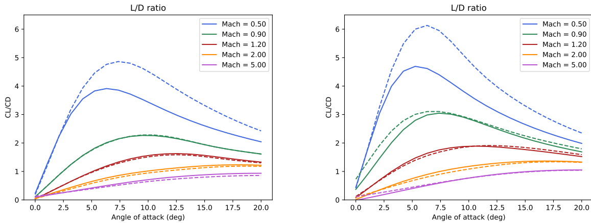
Figure 10: Lift over Drag ratio between NACA (dash line) and double-wedge (solid line) airfoil profiles, as a function of Mach number and angle of attack. Two configurations are evaluated: wingspan equivalent to three times the stage diameter (left), wingspan equivalent to five times the stage diameter (right).
