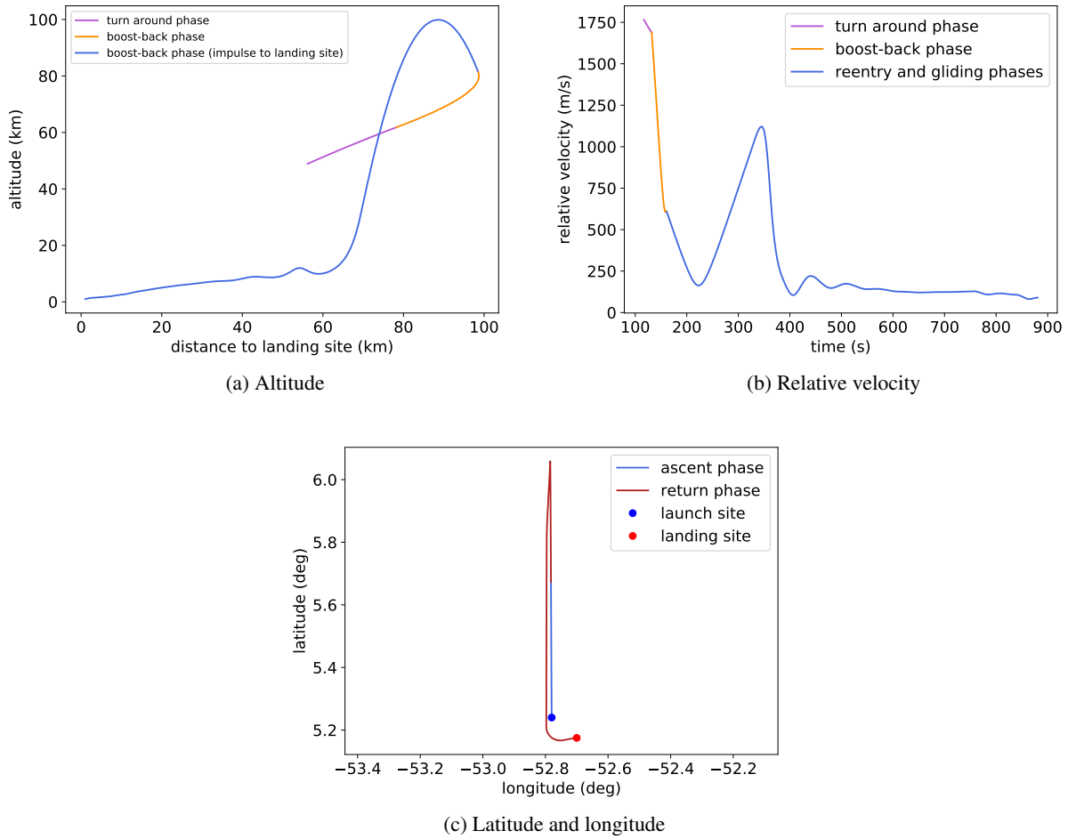
Figure 13: Illustration of generic return trajectory: altitude as a function of distance to the landing site, relative velocity as a function of time, and latitude as a function of longitude
