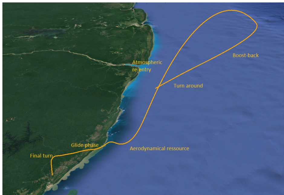
Figure 6: Illustration on the different maneuvers during the RTL phase
