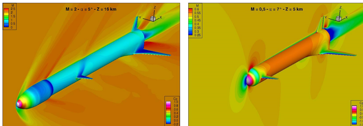
Figure 4: Illustration of CFD RANS calculations: full configuration in supersonic flight (left) and first stage configuration in subsonic glide (right)
