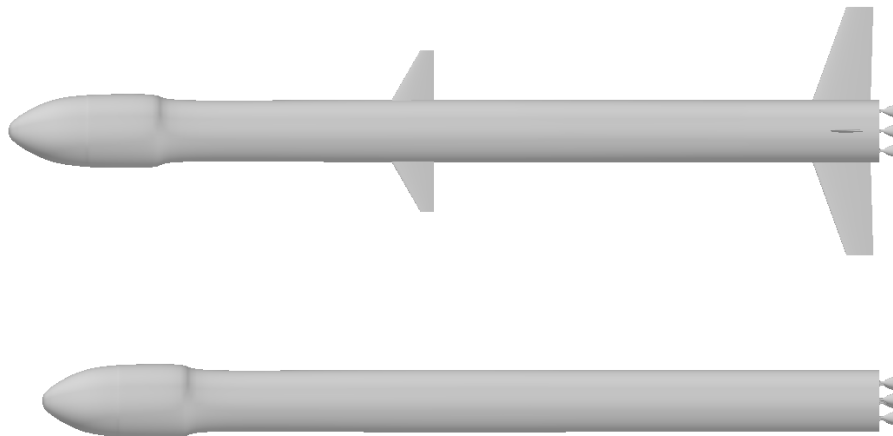
Figure 1: Expendable baseline (bottom) and reusable configuration (top)
