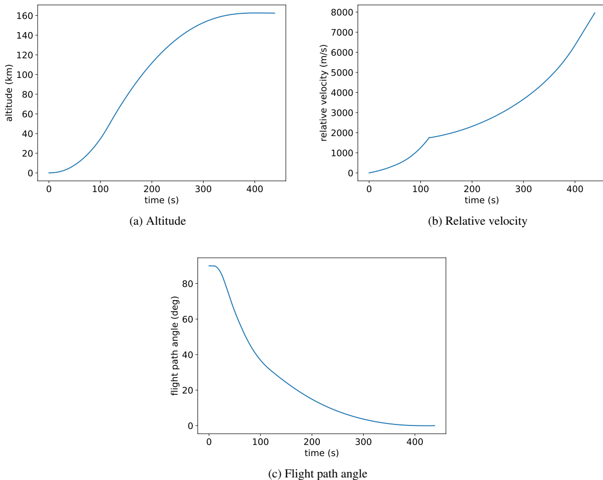
Figure 12: Illustration of altitude, velocity and flight path angle as a function of time for the ascent propelled phase
