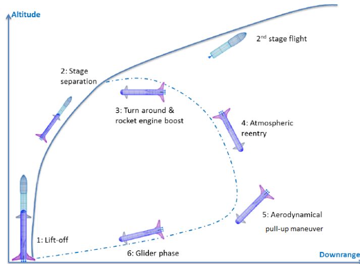
Figure 5: Ascent phase and RTLS by glide-back strategy
