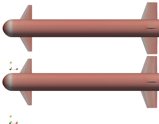
Figure 9: Pressure fields (CFD Euler calculations) for two studied configurations (up: symmetrical NACA, bottom: double-wedge) at subsonic regime (Mach number: 0.5, angle of attack: 5 deg)
