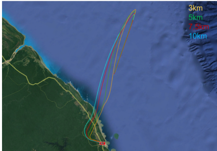
Figure 15: Illustration of the sensitivity study to the radius of the terminal turn (yellow: 3km, green: 5km, red: 7.5km, blue: 10km)
