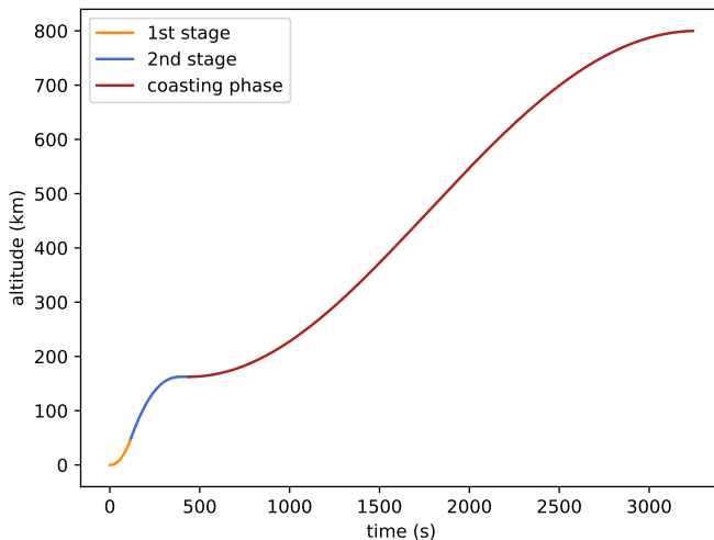
(a) Illustration of the ascent trajectory, altitude as a function of time
