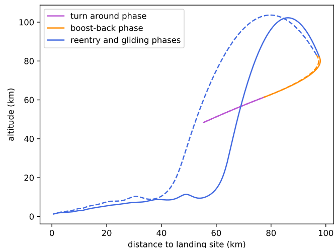
Figure 16: Illustration of return trajectories for the two airfoil profiles described in Section 4.1, altitude as a function of the distance to landing site (in solid line: NACA airfoil profile, in dash line: double-wedge airfoil profile)
