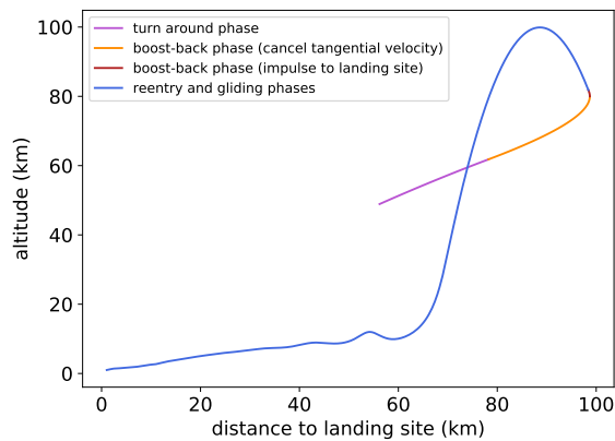
Figure 14: Illustration of the return trajectory, with the different propelled (decomposed into the inversion of horizontal velocity in orange and impulse to the landing site in red) and non propelled phases
