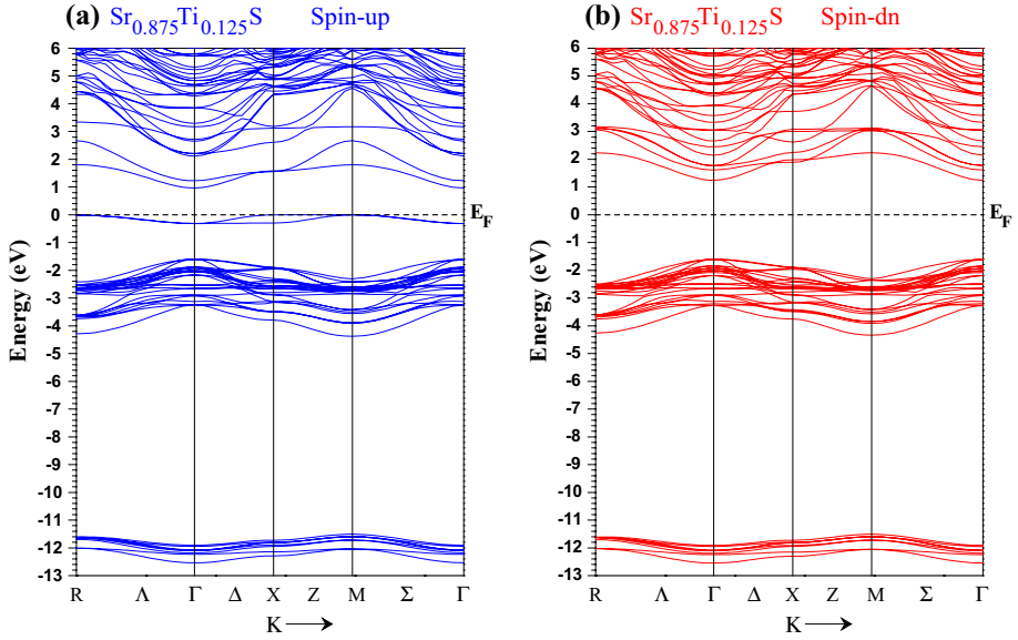
Fig. 2 Spin-polarized band structures for \text{Sr}_{0.875}\text{Ti}_{0.125}\text{S} . a Majority spins (up) and b Minority spins (dn). (Fermi level ( E_F ) is set to zero)
