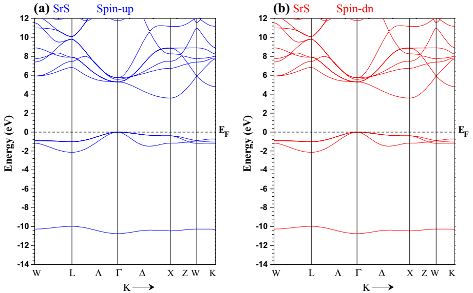
Fig. 1 Spin-polarized band structures for SrS. a Majority spins (up) and b Minority spins (dn). (Fermi level ( E_F ) is set to zero)
