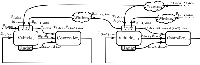
Fig. 2. Block diagram of the platoon system with a PCACC control between vehicle i - 1 and vehicle i .
