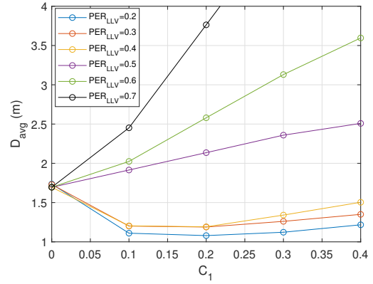
Fig. 4. Illustration of the average inter-vehicular distance with PER_{i,i+1} = 0.0245 for different C_1 values.
