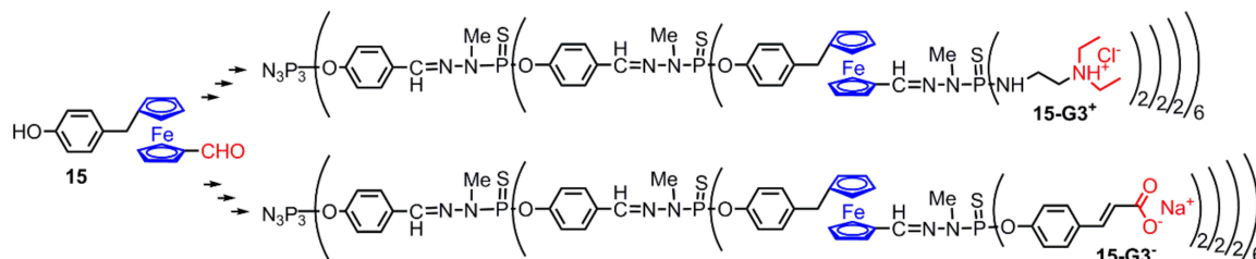
Figure 11. Bifunctional ferrocene 15 used at a single layer of water-soluble dendrimers 15-G3 + and 15-G3 - .
