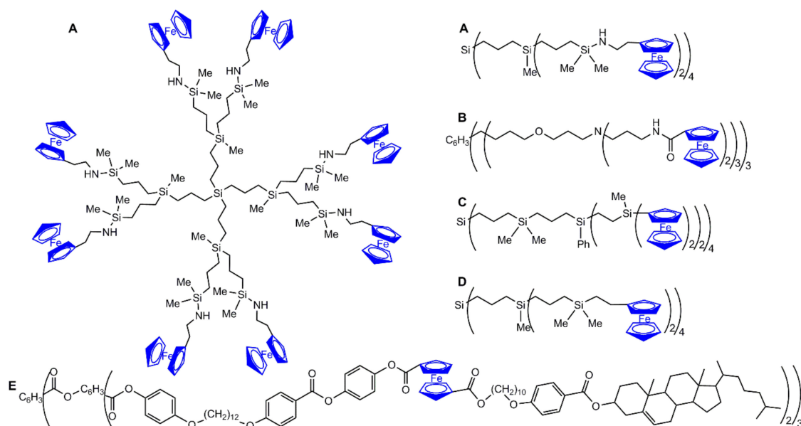
Figure 1. Early examples of ferrocenyl dendrimers. Dendrimer A is drawn two times: the full structure is on the left and the linear structure is on the right. The other dendrimers (B to E) are drawn linearly.
