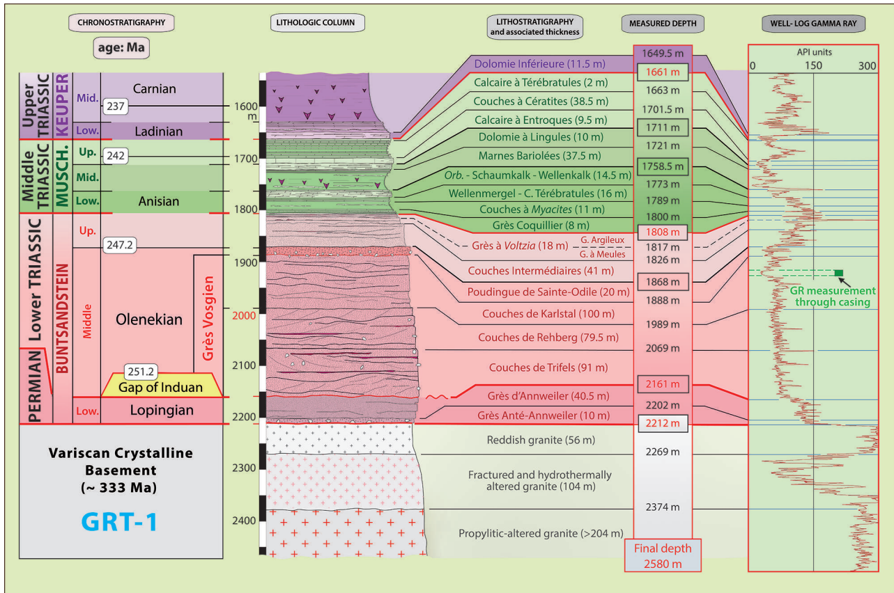
Fig. 6. Complete chrono-lithostratigraphic log of the Muschelkalk, Buntsandstein and granite with the gamma ray log showing all the limits and geological formations encountered in Rittershoffen's well. Orb.: Couches à Myophoria orbicularis ; G.: Grès; C.: Couches; Musch.: Muschelkalk.
