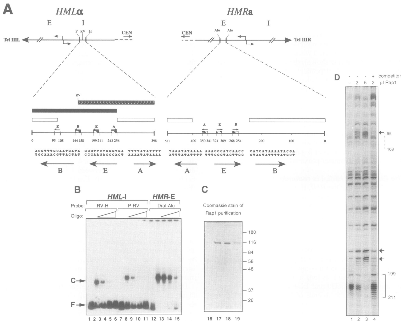
Fig. 4. The minimal HML-I silencer has an ARS consensus and binding sites for Rap1 and Abf1. (A) A comparison of the two silencers HML-I and HMR-E , situated near the telomere of either the left or the right end of the yeast chromosome III, respectively. The top sketch shows the organization of the silent mating type loci on chromosome III. The 398 bp PvuII – HindIII fragment containing I silencer activity from HMLα (left side) and the 521 bp AluI – AluI E silencer from the HMR locus are enlarged in detail. The open bars indicate sequences that are either not necessary or not sufficient to confer repression (Feldman et al. , 1984; Brand et al. , 1987), while the black box indicates the minimal functional HML-I silencer (Feldman et al. , 1984). The stippled box indicates the ΔB silencer fragment ( EcoRV – HindIII ) which we show here to confer significant repression on the LEU2 + lacZ reporter. Within the necessary region of HML-I we indicate the perfect or near perfect consensus for Rap1 (labelled E; see consensus in Figure 5 and Gilson and Gasser, 1995), the binding site for Abf1 (labelled B, based a footprint and the consensus TATCATN5ACGA, Buchman et al. , 1988) or the ARS consensus (labelled A, representing A/TTTTCAT/T A/GTTTA/T). The open box labelled E at HML-I is a slightly less perfect Rap1 consensus (10/13), but which is not essential for full silencer activity. The binding sites indicated at HMR-E are based on Brand et al. (1987), and the sites for the three factors are in nearly identical orientation and spacing to that found at HML-I , in relation to the repressed promoters. Below the map, the actual sequences of the relevant sites are given. At HML-I , these are bp144–158 for the Abf1 or B site; bp 199–211 for the Rap1 or E site; bp 243–256, for the ACS or A site; and at HMR-E , bp 350–341 for the ACS or A site; bp 321–309 for the Rap1 or E site; and bp 268–254 for the Abf1 or B site. Numbering is from the telomere proximal side towards the centromere, based on the Chr. III sequence in the EMBL data base. In vitro footprint assays confirm that Rap1 binds the two indicated sites at HML-I . RV, EcoRV ; H, HindIII ; P, PvuII ; and Alu, AluI . (B) Gel retardation assays were performed using E. coli -expressed and affinity-purified Rap1 protein. The three end-labelled probes used for the assay correspond to the 240 bp EcoRV – HindIII fragment (lanes 1–5) and the 158 bp PvuII – EcoRV fragment (lanes 6–10) of the HML-I silencer, and the 134 bp DraI – AluI fragment of the HMR-E silencer (lanes 11–15). Equivalent moles of each probe were incubated with the same molar excess of Rap1 protein, 0.2 μg of non-specific competitor, and either no specific competitor (lanes 2, 7 and 12) or with 25 ng (lanes 3, 8 and 13), 50 ng (lanes 4, 9 and 14) or 100 ng (lanes 5, 10 and 15) of the 003–004 oligonucleotide containing a telomeric Rap1 site (see Materials and methods). Lanes 1, 6 and 11 contain probes alone, in the absence of Rap1. Protein–DNA complexes were separated on an 0.8% agarose gel (see Materials and methods). 'C' = Rap1–DNA complex; 'F' = free probe. Quantitation shows that the Rap1– HMR-E complex is 4.3-fold more stable than the complex formed with the EcoRV – HindIII fragment and 4.5-fold more stable than the complex formed with the PvuII – EcoRV fragment. (C) A Coomassie blue-stained SDS gel shows the peak elution fractions (lanes 17 and 18) and one fraction before and after these (lanes 16 and 19) from the affinity purification of bacterially expressed Rap1 protein. Molecular weight markers are indicated at the left in kDa. Rap1 is estimated to be 95% pure by this criterion and no major DNA binding contaminant could be detected. (D) DNase I footprint with purified Rap1 protein on the 398 nt ( PvuII – HindIII ) HML-I silencer fragment. Rap1 protein binding to the I-silencer fragment and DNase I digestions were performed as described in Materials and methods. The 398 nt I-silencer fragment (10 ng each) was incubated without (lane 1), with 2 μl (~24 ng, lanes 2 and 4) and with 5 μl (~60 ng, lane 3) of Rap1 protein. Nuclease digestions were performed with 0.1 μg/ml DNase I (lanes 1–4). Digestion products were PCR amplified using the end-labelled oligonucleotide, SG105, and analysed on an 8% polyacrylamide–7 M urea sequencing gel together with dideoxy sequencing products of the 398 nt I-silencer fragment (not shown). The site of Rap1 binding is indicated by a bracket along the autoradiogram, the slightly less perfect Rap1 consensus by a dotted line. The numbers correspond to I-silencer sequences of putative Rap1 binding sites as in (A). Arrows along the autoradiogram indicate DNase I-hypersensitive sites.
