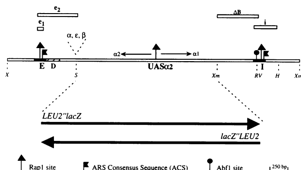
Fig. 1. The LEU2' lacZ reporter constructs used in this study. Top: shown is a diagram of the HMLα locus, indicating the positions of the HML alleles used in this work (see Materials and methods), important restriction enzyme sites, the upstream activating sequence ( UASα2 ), the two \alpha1 and \alpha2 mating type genes, the E and I silencers and the D element (hatched box). The minimal E and I silencers are shown as black boxes and their size (130 and 150 bp, respectively) and localization are according to Feldman et al. (1984). The symbols which represent the Rap1 sites, Abf1 sites and ARS consensus sequences (ACS) are shown at the bottom of the figure. Deletions used in this study are represented as open boxes above the HML diagram. The e1 deletion corresponds to a substitution of 34 nucleotides by a Bgl III linker within E, inactivating both the Rap1 site and the ARS sequence (Mahoney et al. , 1991). The e2 deletion extends e1 until the Spe I site, removing the D element (see Materials and methods). \Delta B corresponds to a deletion of the HML XmnI–EcoRV 592 bp fragment carrying the Abf1 site of I. The \Delta I deletion, or \Delta I^{242} in Mahoney and Broach (1989), is a 280 bp deletion which removes the Abf1 site, the Rap1 site and the ARS sequence. Oligonucleotides corresponding to binding sites for ORC, Abf1 and Rap1 (named respectively \alpha , \beta and \epsilon , see Figure 5) were inserted at the junction between the HML DNA and the reporter gene at the Spe I site. (X) Xba I, (S) Spe I, (RV) EcoRV , (H) Hind III, (Xm) Xmn I. Bottom: the 3.4 kb LEU2' lacZ reporter gene DNA is inserted in place of a 2.1 kb HML Spe I– Xmn I DNA fragment.
