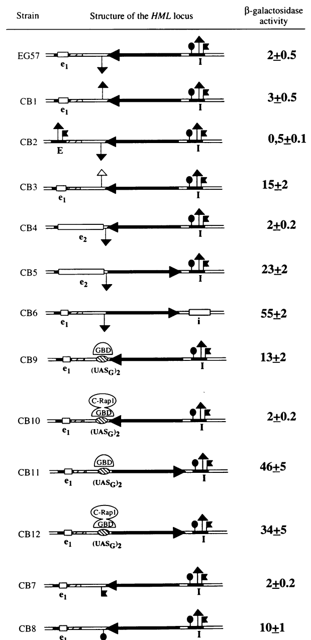
Fig. 6. Cooperative effects between I and individual silencer elements. This figure includes the structure of various LEU2 + lacZ insertions at HML , as well as the name of the strains to the left of the structure and the relative values of \beta -galactosidase produced in the corresponding strain to the right. The symbols are described in Figure 1 and the \beta -galactosidase activity measurements are as previously described, always standardized to the 0.07 Miller units obtained with EG5 and EG31. In every experiment, the EG5 control is performed in parallel and values are reproducibly 0.07 \pm 0.01 . The symbols corresponding to proto-silencers are below the line when the orientation is different from the orientation in the natural HML-E silencer. The triangle which symbolizes a Rap1 binding site is empty in the case of \epsilon' oligonucleotide insertion, which corresponds to a mutated form of a Rap1 site (see Figure 5). All the strains derived from GA210 and are LEU + . The strains with a dimer of Gal4 binding sites [(UAS G ) 2 ] carry a disrupted chromosomal GAL4 gene ( gal4::LEU2 ). CB9 and CB11 contain a low copy number plasmid expressing the Gal4 DNA binding domain (GBD) and CB10 and CB12 contain a low copy number plasmid expressing a hybrid protein between GBD and aa 653–827 of Rap1.
