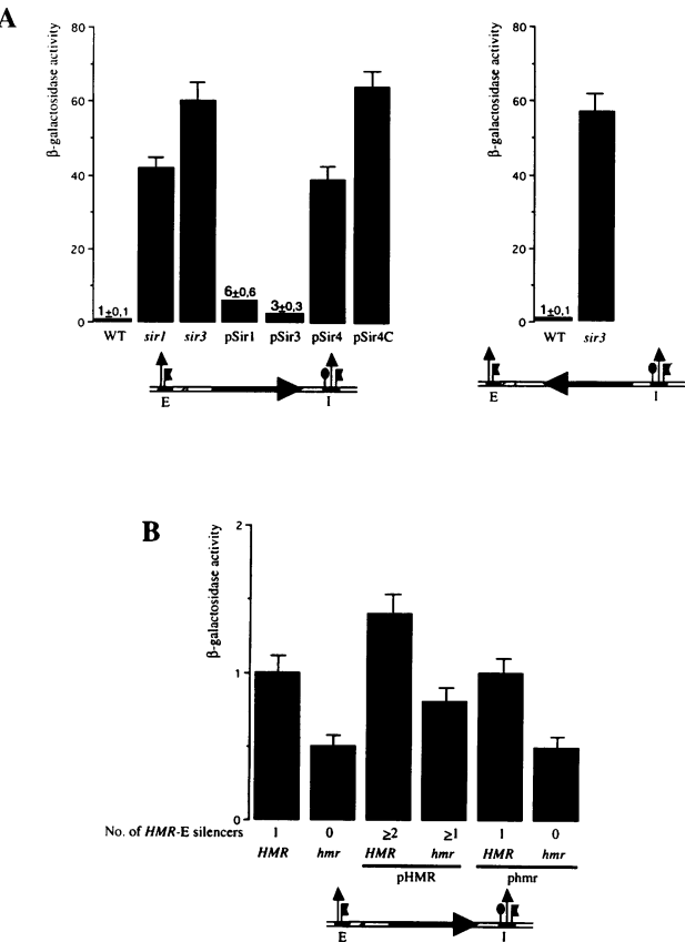
Fig. 2. LEU2' lacZ expression at the HML locus requires Sir proteins and is sensitive to the dosage of repressed domains. The relative \beta -galactosidase activities produced in yeast strains carrying a LEU2' lacZ reporter gene inserted between the E and I silencers at the HML locus are indicated in the bar graph. The structure of the HML region in the assayed strains is indicated below each diagram. The symbols are as in Figure 1. Strains with the reporter gene in either orientation according to the E and I silencers produced the same amount of \beta -galactosidase activity (0.07 Miller units, see Materials and methods) which was standardized as 1 (strain EG5, left diagram in A and B and strain EG33, right diagram in A). The error bars represent the standard deviation of the mean, calculated from the results of at least four independent trials; in most cases, the standard deviation did not exceed 10%. To avoid effects of leucine control, all strains were made LEU + by transformation and were grown in the absence of leucine. (A) LEU2' lacZ repression depends on silencing factors. Strains lacking Sir proteins ( sir1 , sir3 ) or strains carrying multicopy plasmids carrying the genes encoding Sir1 (p Sir1 ) or Sir3 (p Sir3 ), Sir4 (p Sir4 ) or the C-terminal third of Sir4 (p Sir4C ) are indicated. WT: wild-type for known silencing factors. Control strains carrying the vectors without inserted SIR genes produced the same amount of \beta -galactosidase as the corresponding WT strain (data not shown). For strains with a low level of expression, the actual numerical values are indicated. (B) The \beta -galactosidase activities according to the number of repressed HMR-E sequences in the cell. hmr indicates that the HMR-E region has been deleted (see Materials and methods). The number of HMR-E silencers present in each cell is indicated below each column, assuming that the copy number of the centromeric pHMR is one per cell. Beneath each column, the relevant strain characteristics and any additional plasmids in that strain are given.
