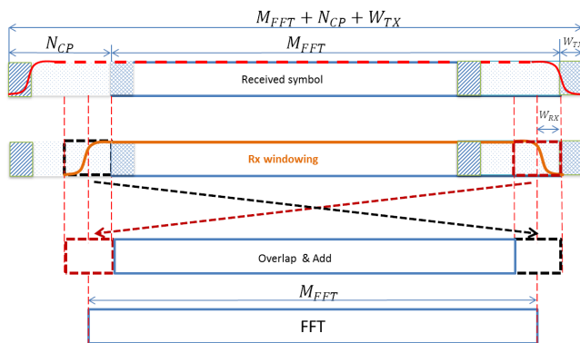
FIGURE 4. WOLA-OFDM processing.
