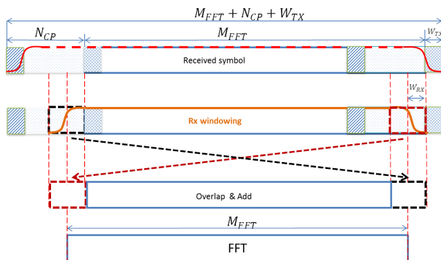
FIGURE 4. WOLA-OFDM processing.
