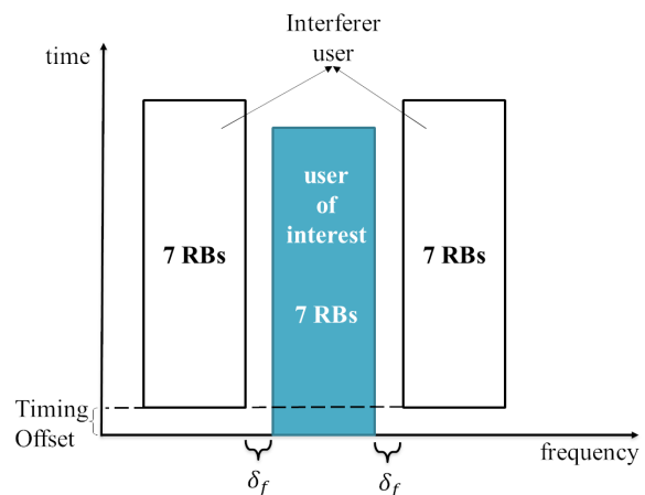
FIGURE 8. Asynchronous scenario.
