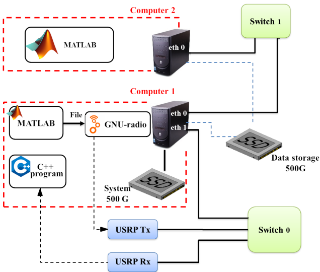
FIGURE 2. Computer architecture.
