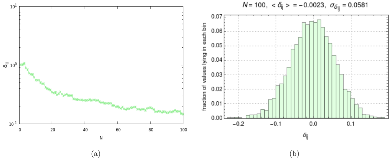
FIG. 1: A scatter plot showing the variation of maximum value of \delta_{ij} of the type LL/RR with respect to number of hidden sectors, N at the high scale (left side). A histogram of the \delta_{ij} is presented. As expected the mean is very close to zero and the variance is as computed in the text.
