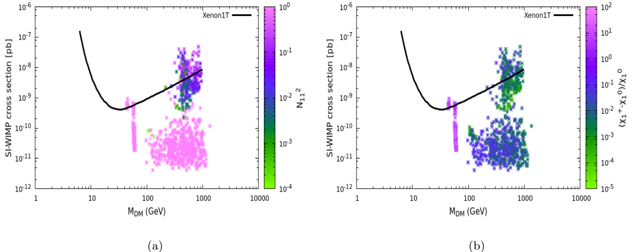
FIG. 4: Regions of the parameter space which satisfy the relic density and the direct detection results from Xenon 1T. On the left we have shown the spin independent cross-section with respect to the lightest neutralino mass and the Bino component of the lightest neutralino. On the right, we show the same, with the mass difference between chargino and Bino.
