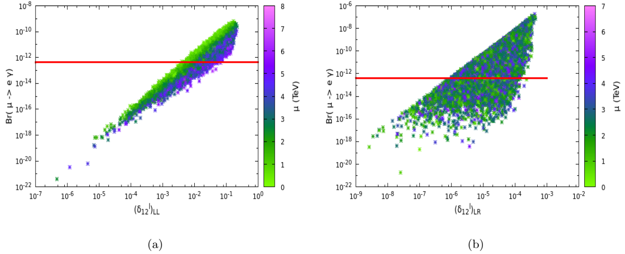
FIG. 3: Regions of the parameter space constrained by the leptonic rare decay \mu \rightarrow e + \gamma for (\delta_{12})_{LL} (on the left) and for (\delta_{12})_{LR} (on the right). The horizontal (red) line is the present experimental limit from MEG experiment. As can be seen, a large part of the parameter space survives the experimental limit for N=100 .
