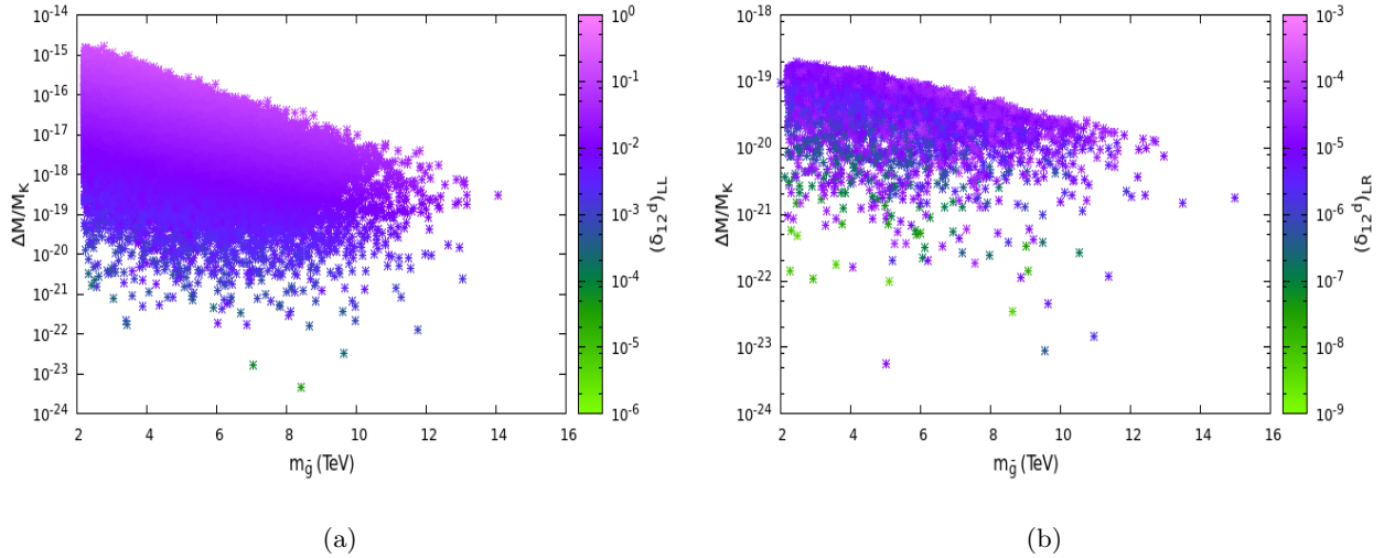
FIG. 2: Regions of the parameter space which satisfy the bounds from LHC, Higgs mass and other phenomenological bounds. We have chosen N to be 100 and \tilde{m} to be 20 GeV. The distribution of \delta values is as per the Eqs. (27) and (32). The left side plot is for LL type mass insertion whereas the right hand side is for LR type mass insertion. All points satisfy the experimental constraint from \Delta M_K .
