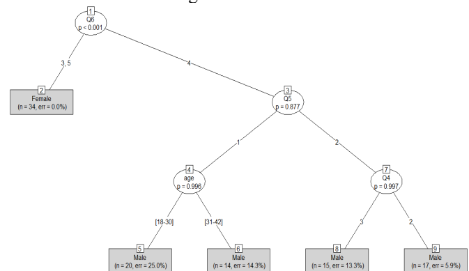
Figure 3. Tree 1
