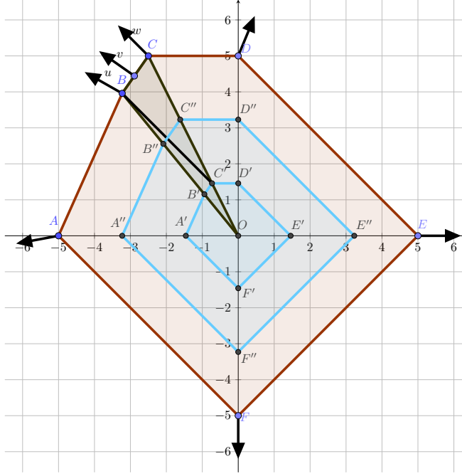
Figure 7: A = (-5, 0) , B = \left(-\frac{5}{3} - \frac{25}{16}, \frac{10}{3} + \frac{5}{4}\right) , C = \left(-\frac{5}{2}, 5\right) , D = (0, 5) , E = (5, 0) , F = (0, -5) . All normals are chosen to be bisectors except w which is parallel to the line (DE) . The vector v is orthogonal to the segment [BC] . The point C' is obtained by considering the intersection between the line (Bw) (starting from B with direction w ), and the segment [OC] . The points A' , B' , D' , E' , F' are obtained by performing a scaling of A, B, D, E, F of a factor \frac{OC'}{OC} . The polygon A''B''C''D''E''F'' is ABCDEF scaled by a factor \frac{OC'+OC}{2OC} .
