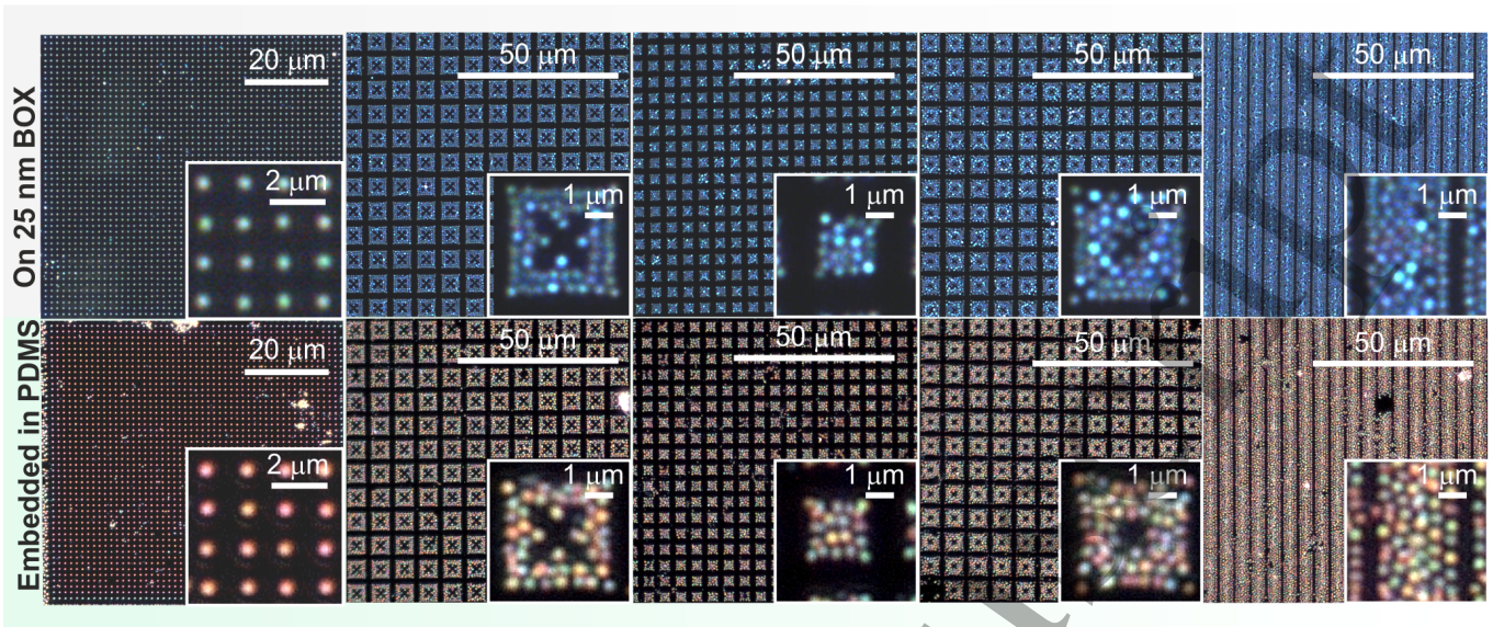
FIG. 6. “Method B, transfer of Si islands obtained by templated dewetting”. Top panels: dark-field optical microscope (100 \times magnification, NA = 0.75) of monocrystalline Si islands on 25 nm BOX. From the left to the right, panels are illustrated with several islands organization obtained from different initial patch size and shape. 31,35 Bottom panels: same as the top panels for islands transferred in a PDMS slice.
