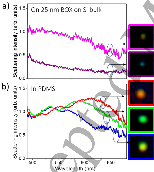
FIG. 7. “Dark-field spectroscopy of individual islands”. Top panel: dark-field resonant scattering spectra of two individual islands on BOX. The top insets (1.5 \mu m side) show the corresponding dark-field microscope images collected at 50 \times . Bottom panel: same as for the top panel but for particles in PDMS.
