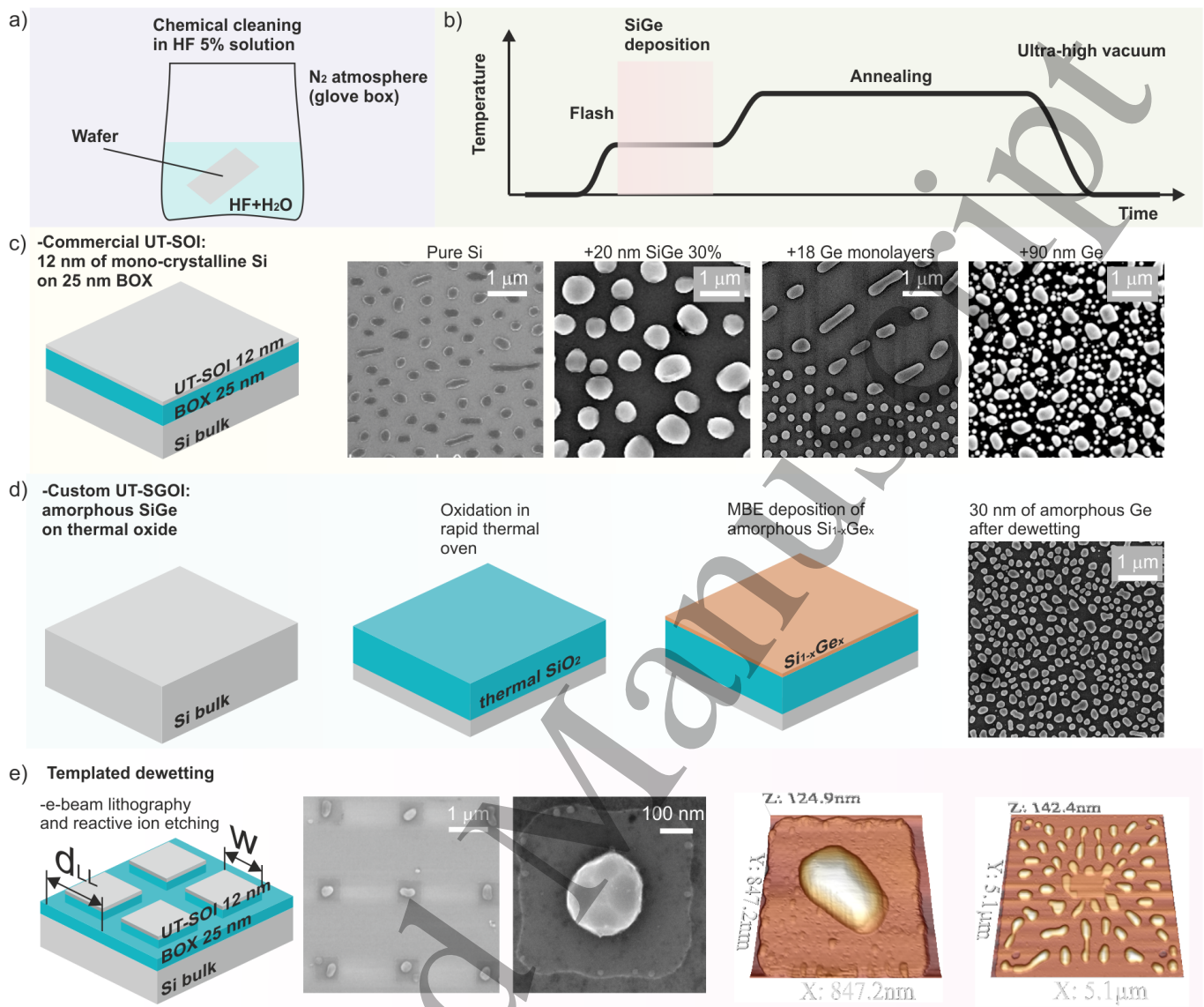
FIG. 1. Solid state dewetting of SiGe alloys and dewetting scenarios. a) Ex situ chemical cleaning of the sample in a glow box under N_2 atmosphere. b) Annealing and deposition cycles in the molecular beam epitaxy reactor (MBE): annealing flash, deposition of SiGe, high temperature annealing to induce the dewetting. c) Commercial ultra-thin silicon on insulator (first panel) can be dewetted to produce monocrystalline, pure-Si islands (second panel), 27 first topped with Si_{1-x}Ge_x alloys and then annealed to produce large SiGe-based islands (third panel), first partially dewetted and then topped with Ge to form bimodal distribution of spatially-separate Si rich and Ge-rich islands (fourth panel), 30 or annealed during Ge deposition to produce bimodal spatially-mixed large and small islands. 33 d) Custom silicon-germanium on insulator can be produced starting from a Si wafer (left panel), oxidation in a rapid thermal annealing oven (second panel), MBE deposition of Si_{1-x}Ge_x alloys (third panel) and dewetting (fourth panel). e) Patterning prior to annealing (e.g. via e-beam lithography and reactive ion etching, first panel) allows to form ordered arrays of Si islands (second to fourth panel) and complex nano-architectures (fifth panel). 27,29,31,34,35
