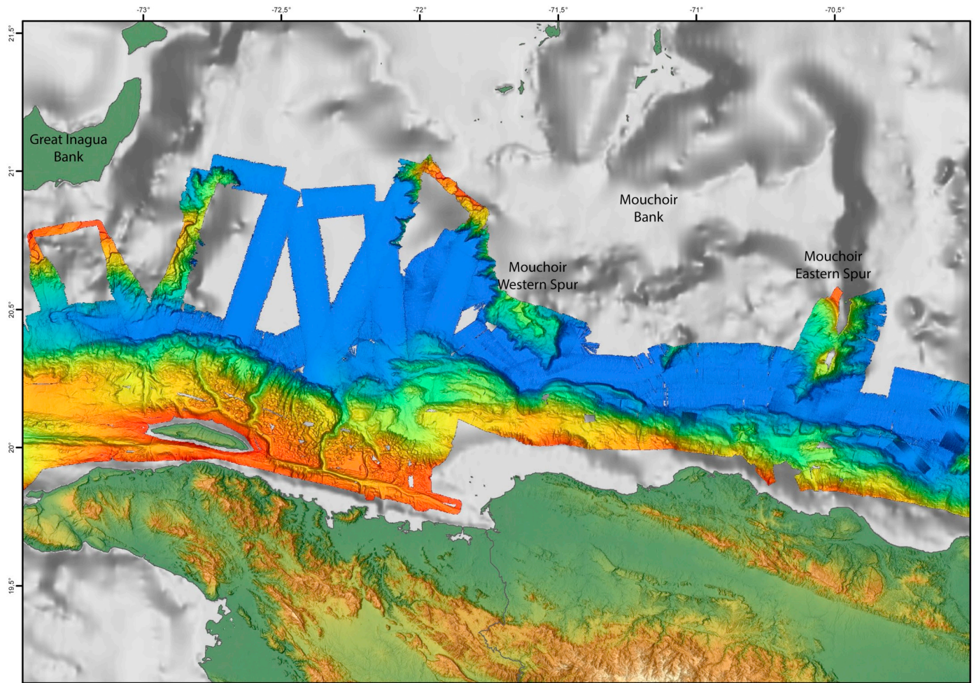
App. C. DEM of the OUD derived from the multibeam bathymetry data and completed with data from GEBCO and SRTM datasets (Weatherall et al., 2015; Farr and Kobrick, 2000). Same data extent as Fig. 10.
