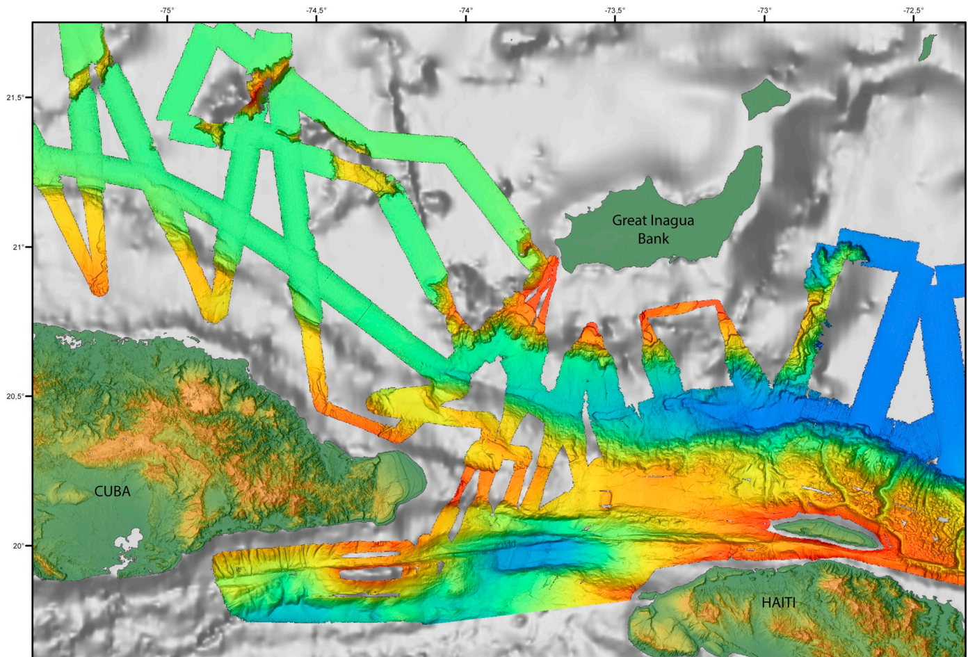
App. D. DEM of the SSD derived from the multibeam bathymetry data and completed with data from GEBCO and SRTM datasets (Weatherall et al., 2015; Farr and Kobrick, 2000). Same data extent as Fig. 14.
