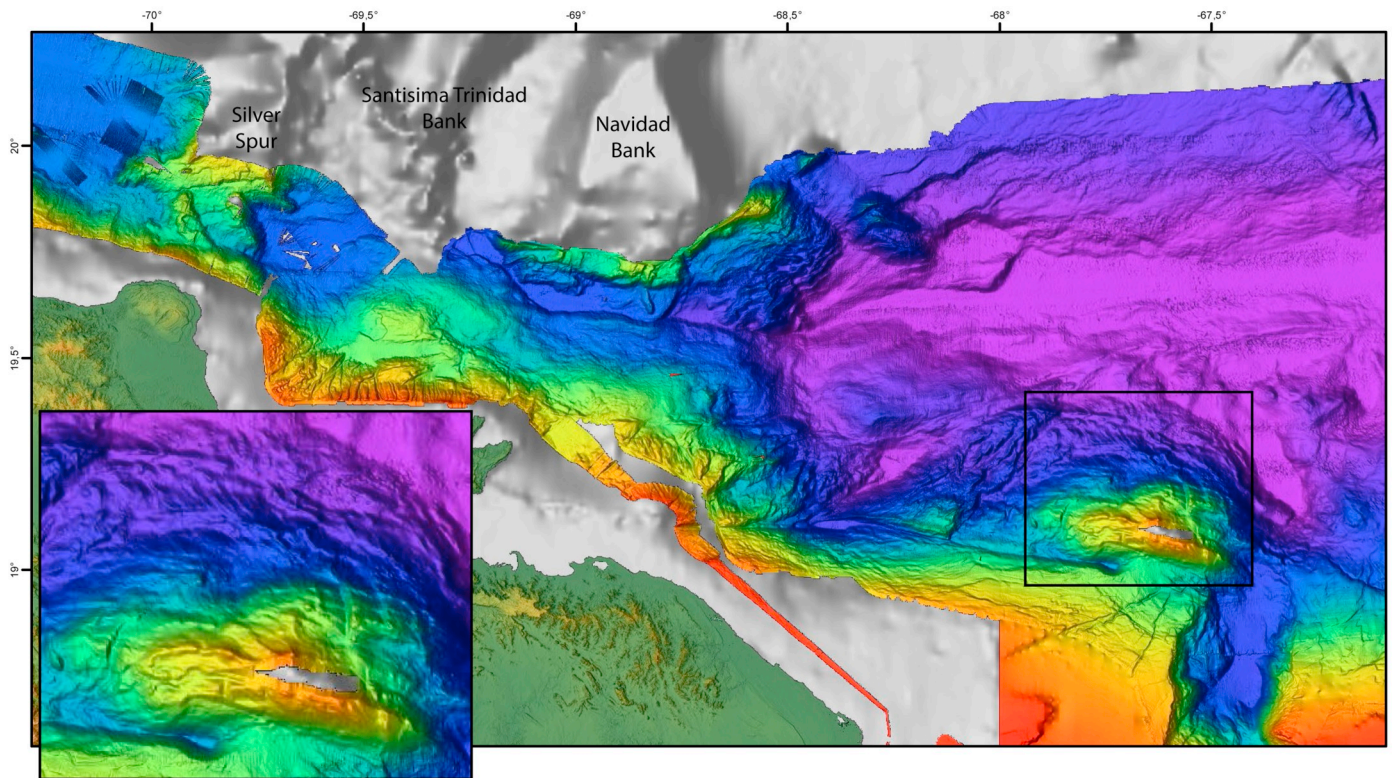
App. B. DEM of the OSD and the OCD derived from the multibeam bathymetry data and completed with data from GEBCO and SRTM datasets (Weatherall et al., 2015; Farr and Kobrick, 2000). Same data extent as Fig. 4.
