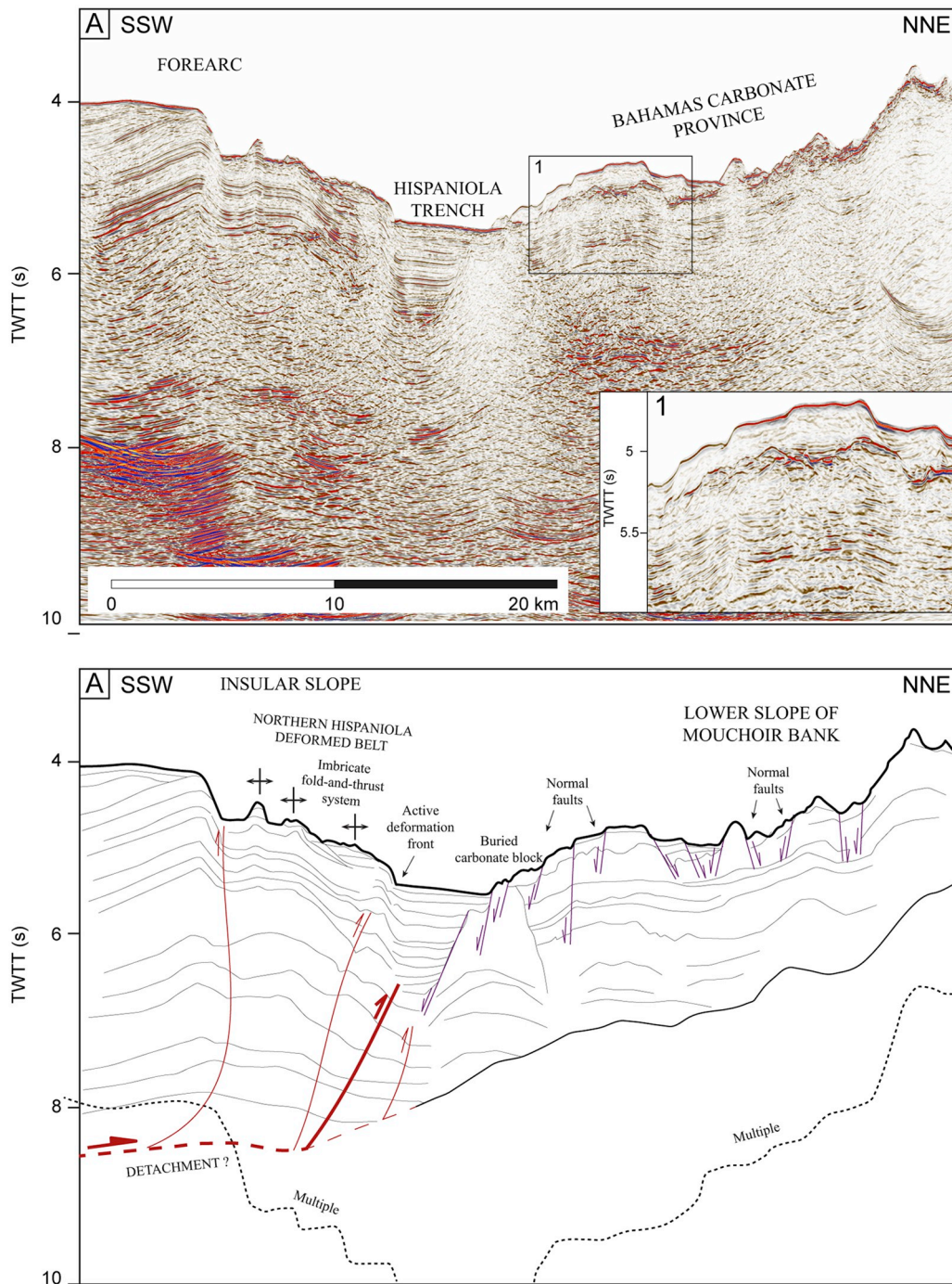
Fig. 12. A) Pre-stack migrated MCS profile. See location in Figs. 2 and 10. V.E. is 6× on the seafloor. B) Line drawing interpretation. See legend in Fig. 5. Inset 1 shows a zoom of the highly faulted BCP blocks.
