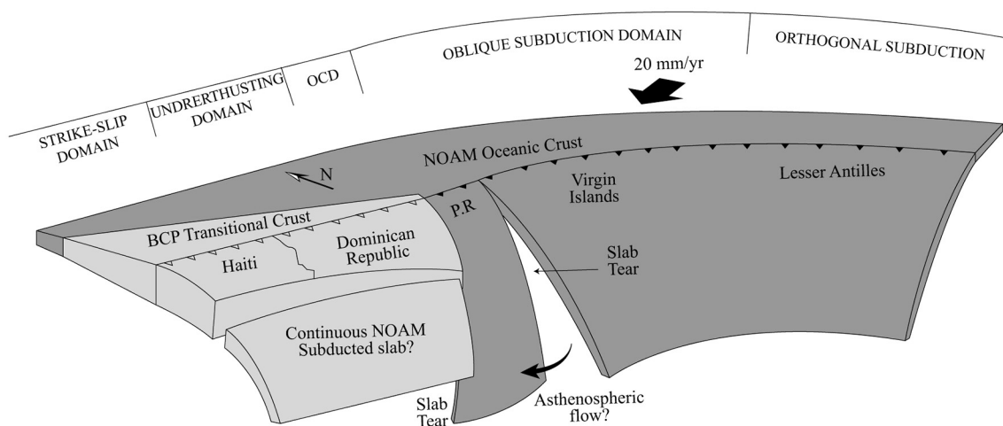
Fig. 19. 3-D view of the proposed geometry for the NOAM slab in the northeastern NOAM-CARIB plate boundary. PR: Puerto Rico.
