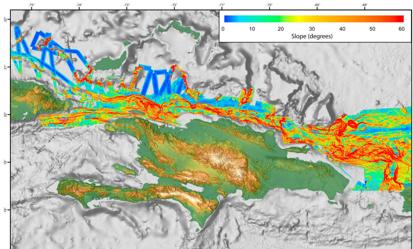
App. A. Gradient map (degrees) of the study area derived from all multibeam bathymetry datasets. See legend for color interpretation.
