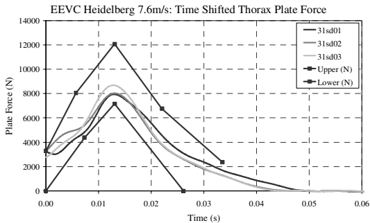
Figure 24: 6.8m/s Heidelberg thorax force EEVC.
