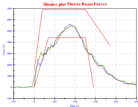
Figure 19. WSU 8.9 m/s padded shoulder and thorax force.
