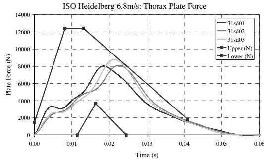
Figure 23. 6.8m/s Heidelberg thorax force ISO.
