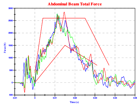
Figure 25. Abdomen force 6.8 m/s rigid WSU.
