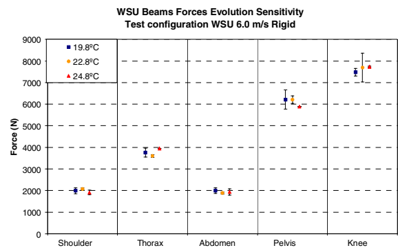
Figure 34. Temperature variation external measurements variability.
