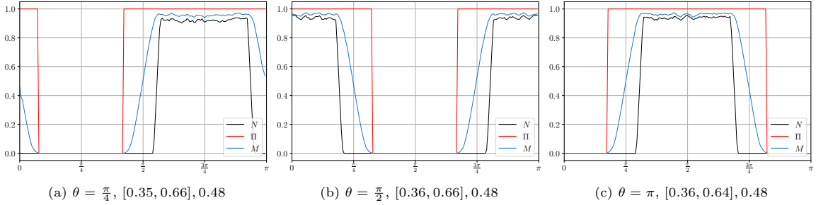
Figure 9: Behavior of surrounding profiles and evaluations with Fuzz-DELS for different rotations of the objects from the configuration (b) of Fig. 5.
