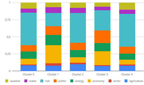
Fig. 13. Composition of the extracted clusters in regard of the taxonomy
