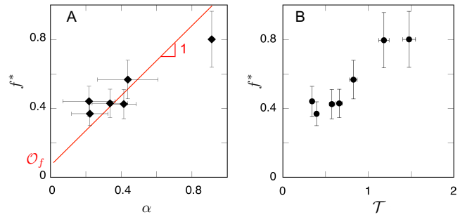
FIG. 4: Fraction f^* = f(t^*) of algae escaped from the foam at t = t^* as a function of the initial slope \alpha = (df/dt)/(dV/dt)|_{t=0} (panel A), and as a function of the escape time number \mathcal{T} (panel B), where \mathcal{T} \propto U is given by Eq. 3. The red line in panel A corresponds to the relation f^* \simeq \alpha + \mathcal{O}_f (see text), where \mathcal{O}_f is an offset taking into account the fraction of CR cells escaped by diffusion. The best fit of the data gives \mathcal{O}_f = 0.08 \pm 0.05 .
