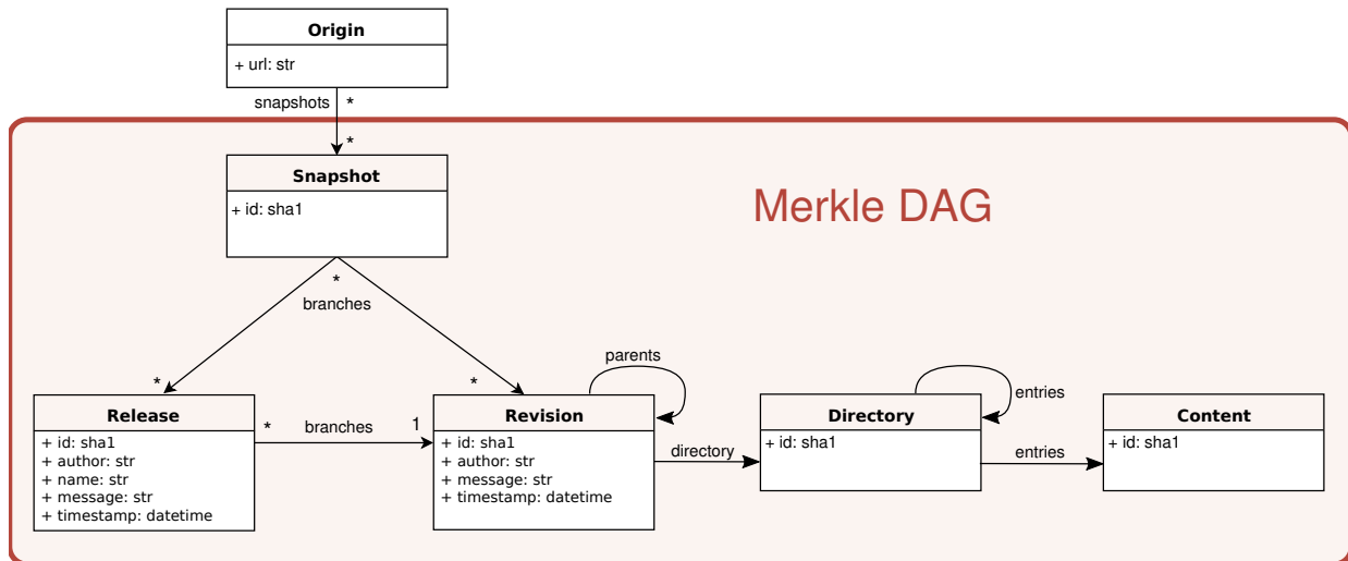
Fig. 1: Topology of the Software Heritage Merkle DAG, which captures software source code together with its full development history.
