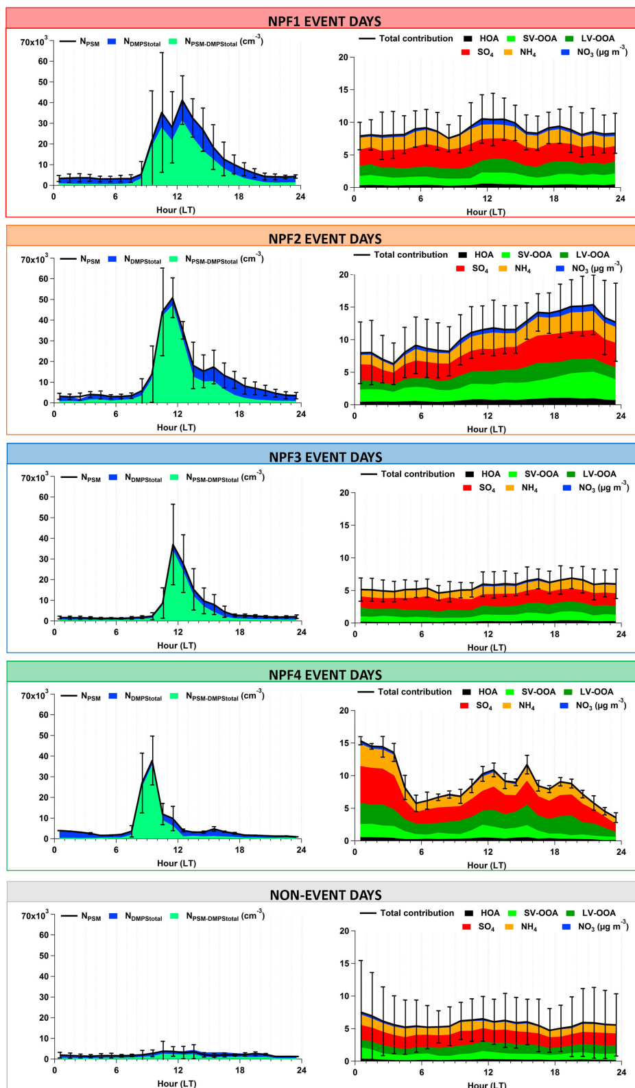
Figure 9. Diel variation of particle number N_{PSM} and N_{DMPS} and accumulated diel variations of PM_{10} contribution for NPF event days (NPF1–NPF4) and non-event days. Diel variations are represented by daily mean values associated with standard deviation when several days were combined. Time is given in local time (UTC+2h).
