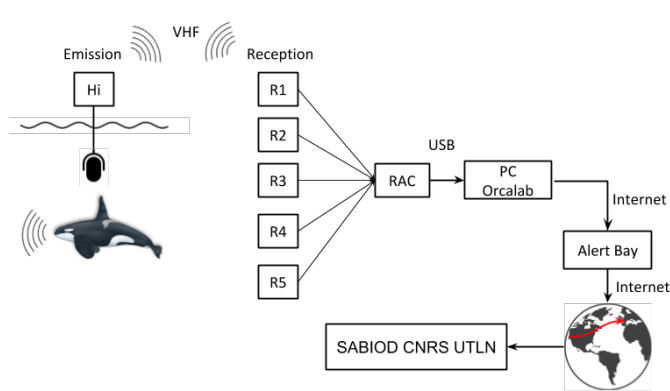
Figure 2. Representation of the data acquisition, from recording until storage on SABIOD CNRS UTLN server.
