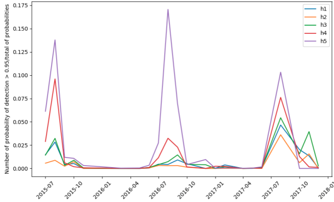
Figure 5. Proportion of two-minute recordings with detected orca calls per month and hydrophone, from 2015 to 2017.
