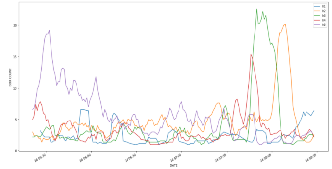
Figure 6. Evolution of the number of detected orca acoustic events from 5:30 to 8:30 am on August 24, 2017
