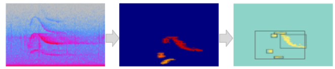
Figure 3. Main steps for the acoustic events extraction: Binarization and detection of connected components. The spectrogram shows frequencies from 0 to 6.5 kHz during 2.5 s.
