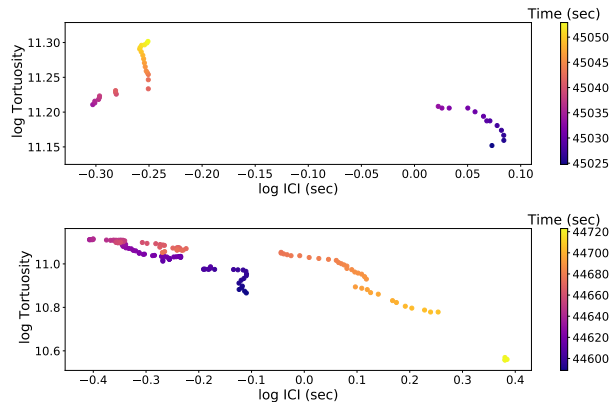
Fig. 7. Scatter plots of log ICI vs. log Tortuosity ( T ). The sequence of 25 sec (Top) shows that the ICI and T are not dependent by construction. The 2 min sequence (Bottom) shows a strong anticorrelation between ICI and T . It could be interpreted as an approach to a prey, a catch (at the minimum of ICI and maximum of T ), and then relaxing ('slack off').
