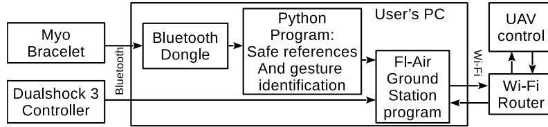
Figure 10: Communication process involved in the armband-UAV interface.
