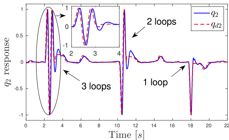
(d) q_2 component, sinusoidal oscillations indicate when a pirouette is performed.
