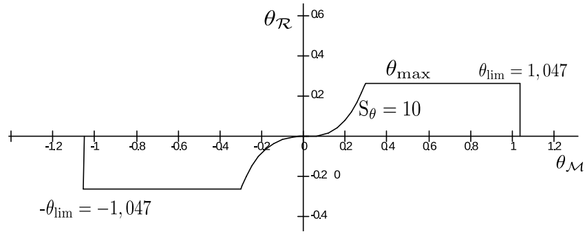
Figure 7: \phi_{\mathcal{R}} with safety limit put in 1.047 rad ( 60^\circ ).
