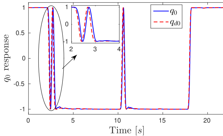
(a) Notice how the sign of q_0 is inverted whenever a loop is performed
