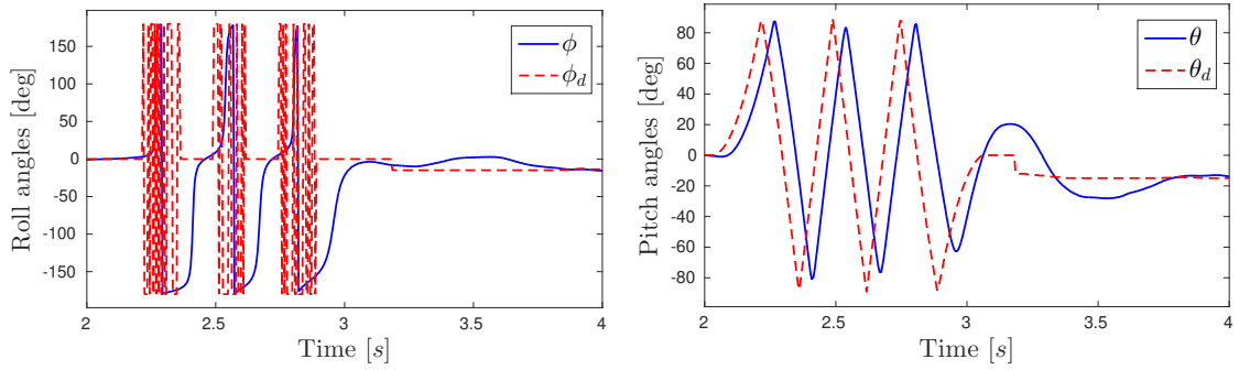
(a) Close up of the \phi euler angle during the triple loop maneuver. Notice the discontinuities in \phi and the Gimball lock in \phi_d .
