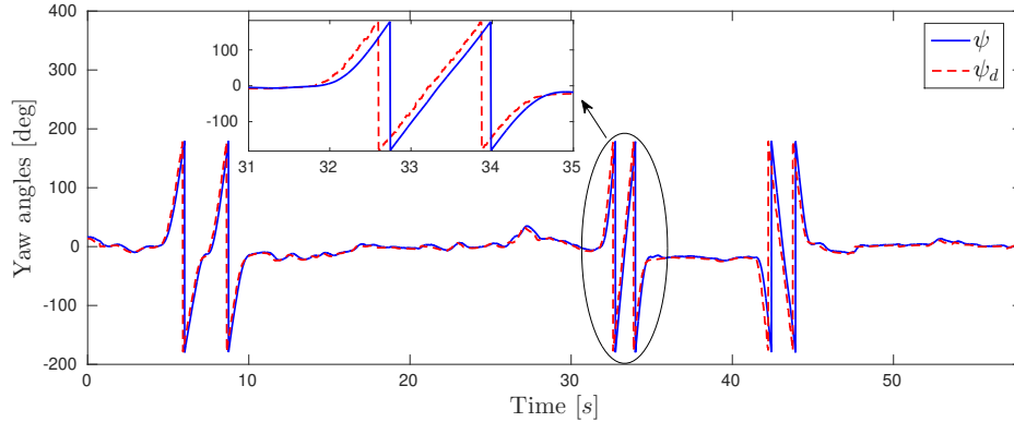
Figure 14: Yaw response using \psi_d from the bracelet. Notice how discontinuities appear in yaw Euler representation when a full 360^\circ turn is performed.
