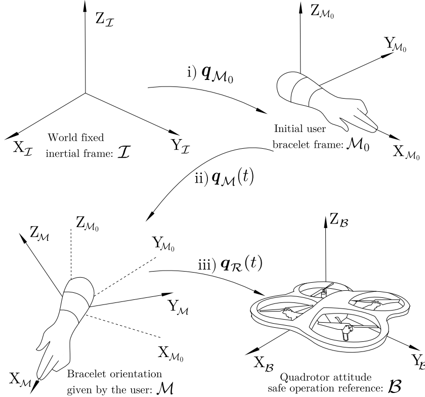
Figure 1: Reference frames for quadrotor attitude reference.
