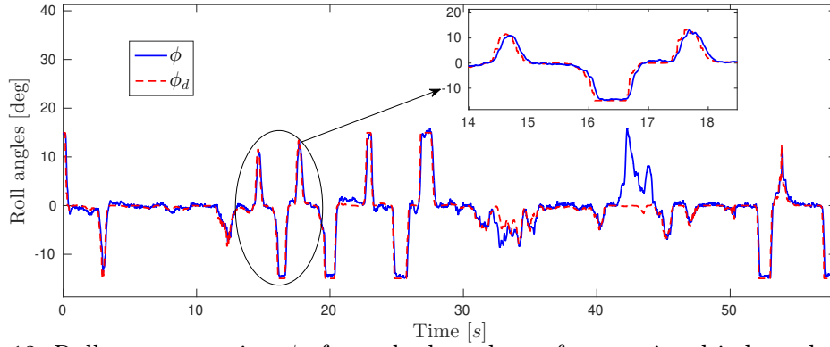
Figure 12: Roll response using \phi_d from the bracelet, reference signal is bounded to safe values between \pm 15^\circ .
