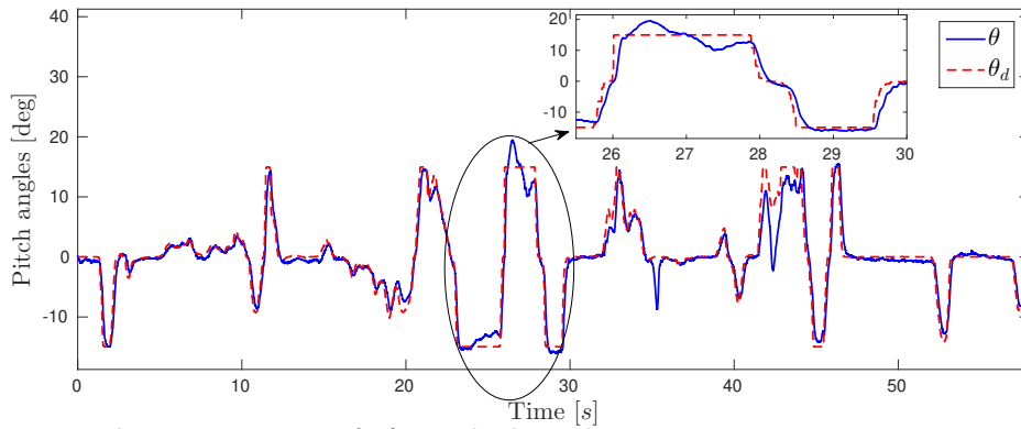
Figure 13: Pitch response using \theta_d from the bracelet, imposing restrictions at \pm 15^\circ values.
