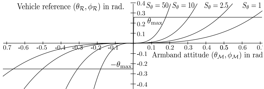
Figure 2: From left to right, greater values \theta_{\mathcal{M}} and \phi_{\mathcal{M}} are required to reach tilt limit a as sensitivity values S_{\theta} and S_{\phi} decrease.
