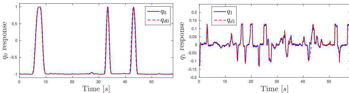
(a) First test q_0 quaternion component, switching its value from -1 to 1 each time a full 360^\circ rotation is performed.
