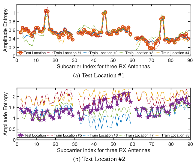
FIGURE 10. Proximity test under (a) LoS condition; (b) NLoS condition.. (a) Test Location #1. (b) Test Location #2.
