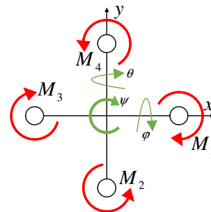
Fig. 2. Quadcopter structure
