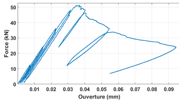
Figure 2. Force-CMOD curve.
