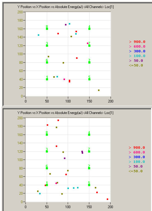
Figure 5: Localization of AE events during primary creep for mortar (a) and concrete (b) in the plan XY.
