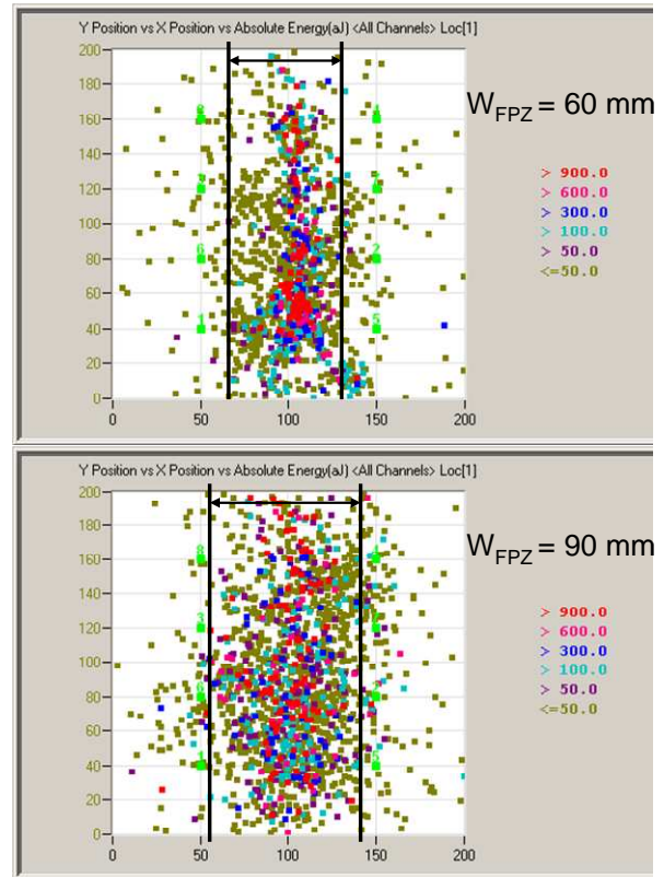
Figure 12: Localisation map of AE events and comparison of the width of the FPZ for mortar and concrete beams.
