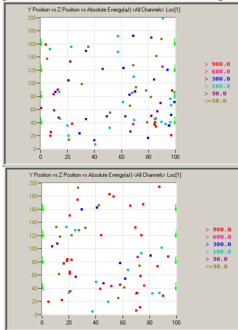
Figure 7: Localization of AE events during secondary creep for mortar (a) and concrete (b) in the plan YZ.
