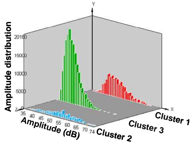
Figure 18: Experimental AE hits amplitude distributions for each cluster
