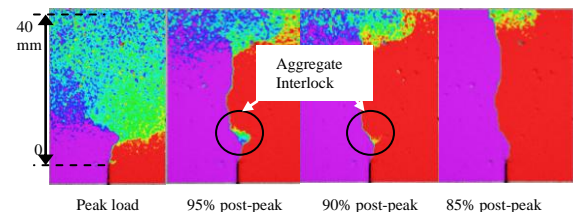
Figure 9: Crack propagation in a specimen showing aggregate interlock.
