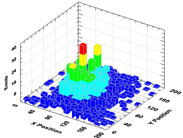
Figure 12: Distribution of AE events on the rectangular grid at final load step
