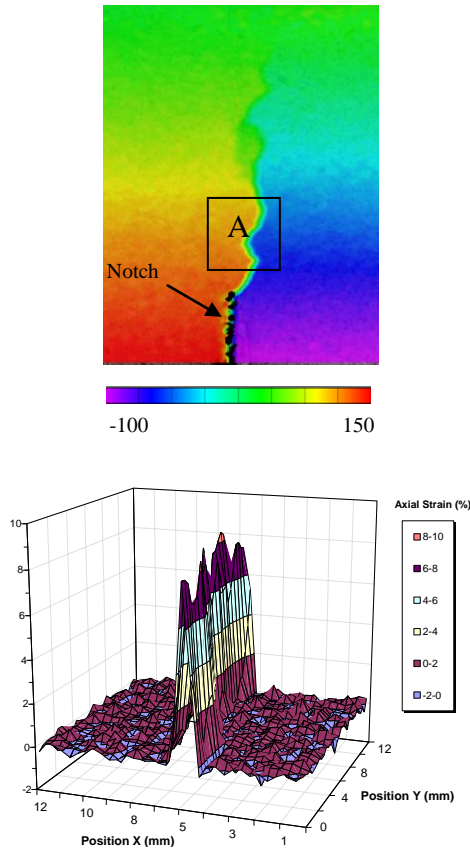
Figure 5: (a) Axial displacement ( \mu\text{m} ) (b) Axial displacement field in the area A.
