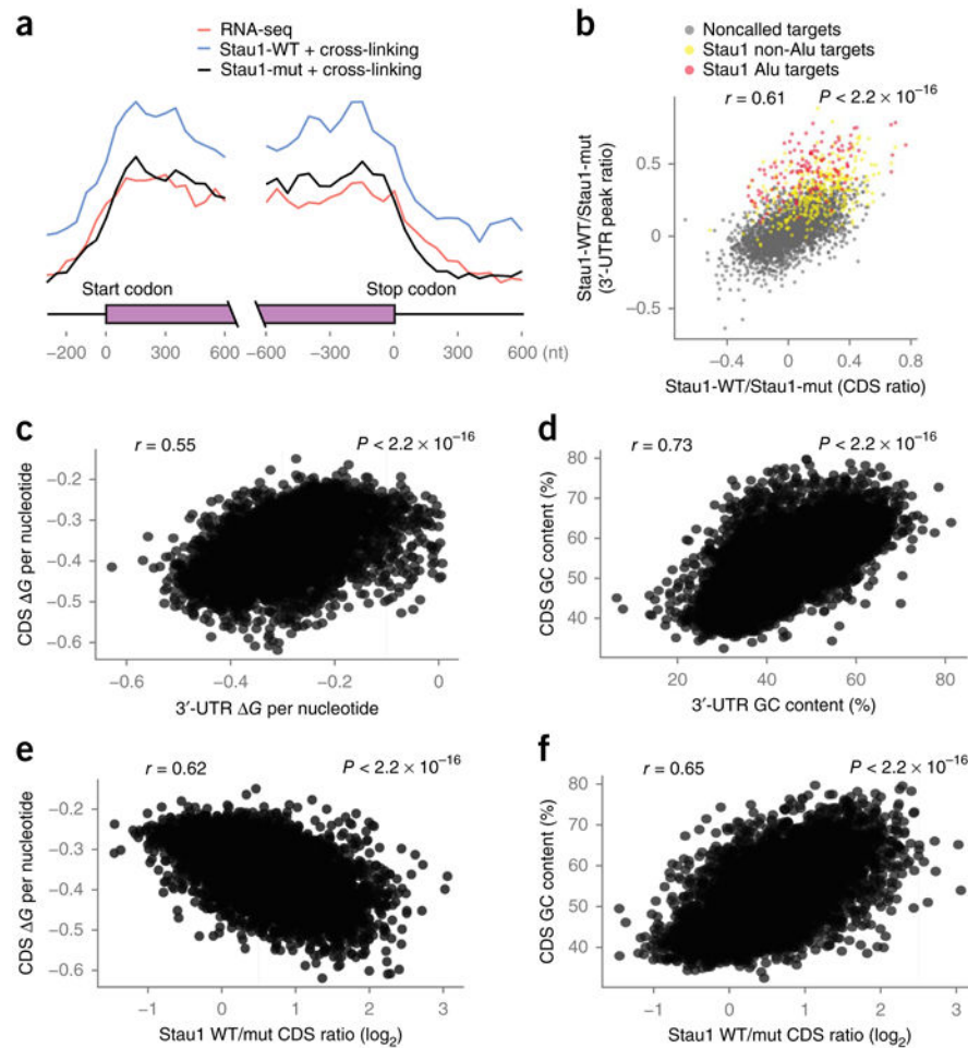
Figure 6. Stau1 occupancy on the CDS strongly correlates with GC content and predicted secondary-structure free energy. (a) Composite plot of the distribution of sequencing reads across the 5' UTR, CDS and 3' UTR of called Stau1-target genes for RNA-seq (red), Stau1-WT CROSS (blue) and Stau1-mut CROSS (black) libraries. (b) Per-gene scatter plot (log 10 ) of total CDS Stau1-WT CROSS read counts/total CDS Stau1-mut CROSS reads counts (CDS ratio) versus the ratio of Stau1-WT CROSS and Stau1-mut CROSS read counts under called 3'-UTR Stau1-WT CROSS peak positions (3'-UTR peak ratio). Red and yellow dots correspond to called Alu- and non-Alu-binding sites, respectively. (c) Per-gene scatter plot of 3' UTR against CDS predicted secondary-structure free energy normalized by the length of the 3' UTR (kcal/mol/nucleotide). (d) Per-gene scatter plot of 3' UTR against CDS GC content (%). (e) Per-gene scatter plot of CDS predicted secondary-structure free energy normalized by the length of the CDS (kcal/mol/nucleotide) against Stau1 WT/mut 3'-UTR ratio (log 2 ). (f) Per-gene scatter plot of CDS GC content (%) against Stau1 WT/mut 3'-UTR ratio (log 2 ). All correlation coefficients and P values were calculated with the Spearman rank correlation (n = 2 biological replicates) throughout figure.
