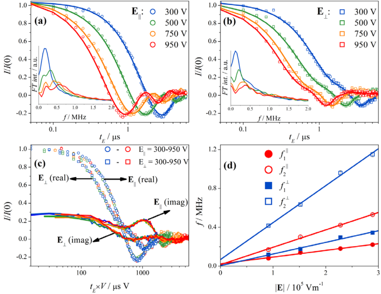
Figure 5. (a), (b) Integrated Hahn echo intensities of the g_{\perp} resonance of \text{Fe}_3 , as a function of the electric pulse intensity and duration, for \mathbf{E}_{\parallel} (a) and \mathbf{E}_{\perp} (b). The lines are fits to exponentially damped oscillations according to the model described in the text. The insets show the FT spectra of the oscillations for the various pulse intensities. (c) In-phase (real) and quadrature (imaginary) signals of the Hahn echo intensities plotted as a function of t_E \times V . The signals collapse into two families depending on the orientation of \mathbf{E} . (d) Oscillation frequencies derived from the fits, plotted as a function of the average electric field intensity; the lines are linear fits.
