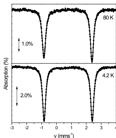
Figure 4. Zero-field Mössbauer spectra of a powder sample of \mathbf{1}_{\text{Td}} at 4.2 and 80 K. Solid lines are theoretical simulations, as described in the text.
