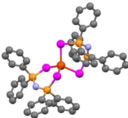
Figure 1. Molecular structure of complex 1Ta . The H atoms are omitted for clarity. Color coding: Iron (brown), selenium (magenta), phosphorus (light brown), nitrogen (blue), carbon (grey).
