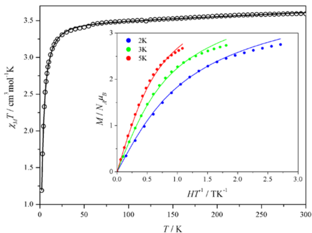
Figure 2. Temperature dependence of \chi_M T of a powder sample of 1Ta under a magnetic field of 1 T. The inset shows isothermal magnetization data plotted as M vs HT^{-1} at the indicated temperatures. Solid lines correspond to the best-fit solution described in the text.
