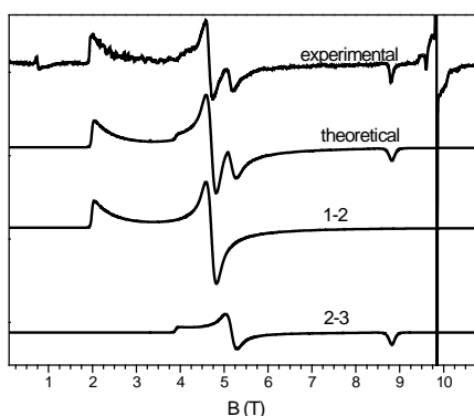
Figure 3. Experimental and theoretical 275.7 GHz cw-EPR spectra of a powder sample of \mathbf{1}_{Td} at 10 K. The theoretical spectra are obtained as described in the text. Experimental conditions: Modulation frequency: 1.8 kHz, modulation amplitude: 3 mT, microwave power: 5 \mu W.
