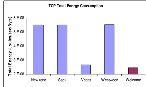
Figure 22. TCP Total Energy Consumption
