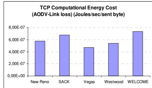
Figure 16. TCP Computational Energy Cost
