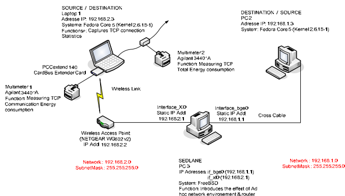
Figure 8. TCP Energy Consumption Measurements Test-bed
