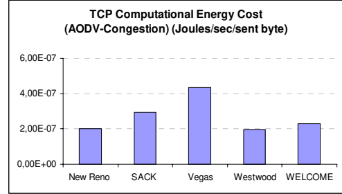
Figure 14. TCP Computational Energy Consumption
