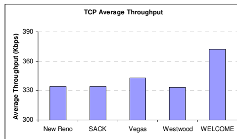
Figure 23. TCP Average Throughput
