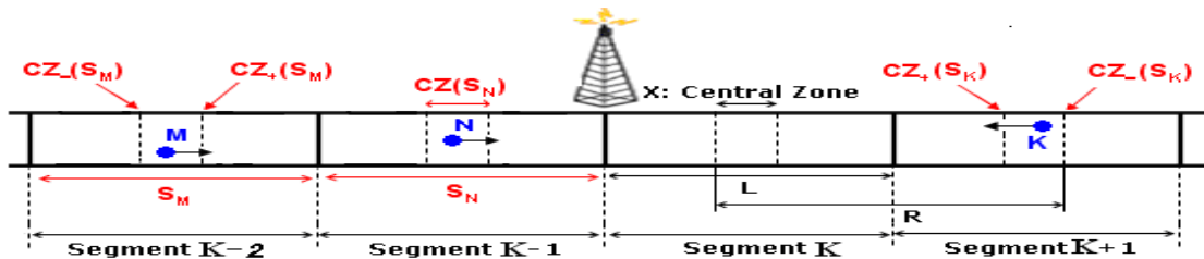
Figure 3. Segment-based architecture
