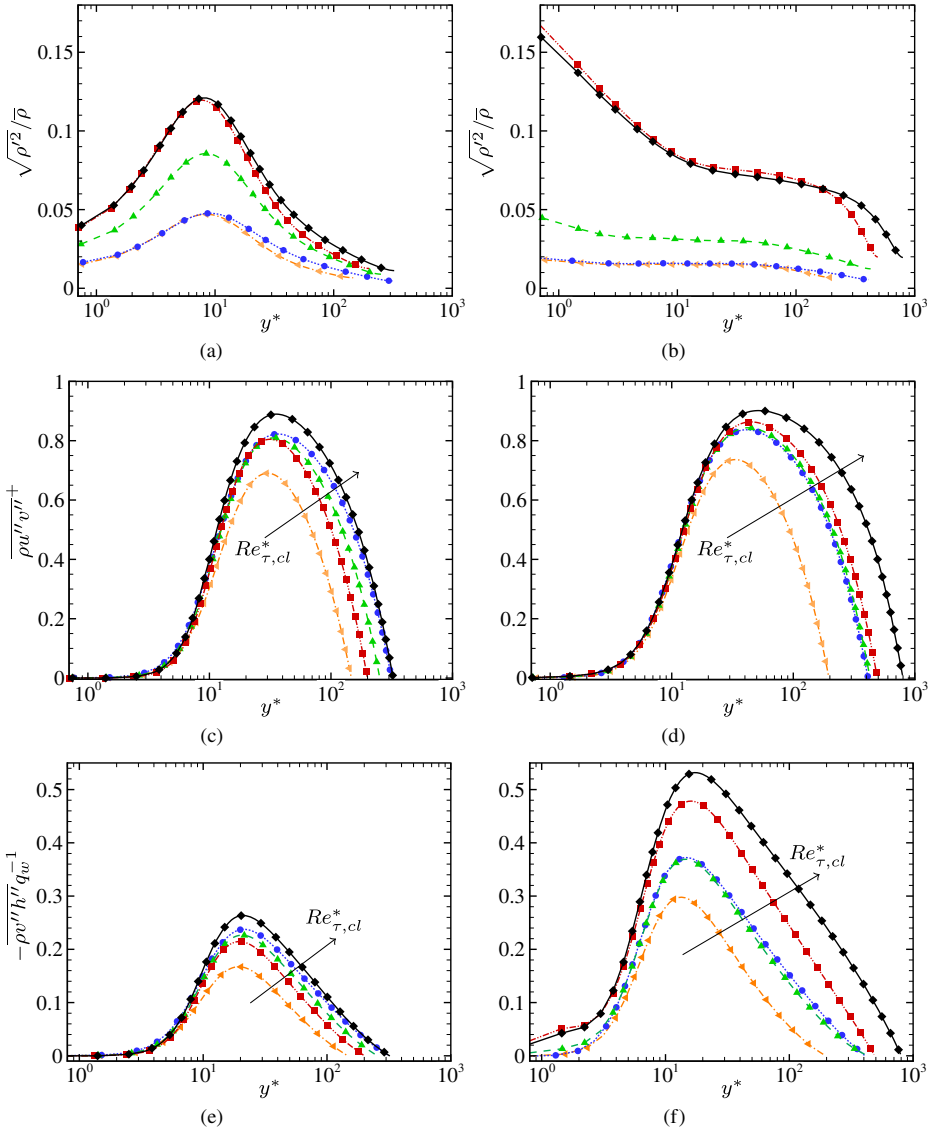
Fig. 6 a, b Normalized density fluctuations ( \sqrt{\rho'^2/\bar{\rho}} ), c, d Reynolds shear stresses ( \overline{\rho u''v''+} ), and e, f profiles of \overline{\rho v''h''} normalized with q_w as a function of y^* for DNS of air (left column) and PP11 (right column) TCF at various M_B and Re_B . Line legend as in Table 3
