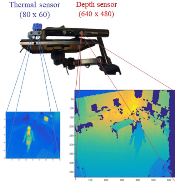
Fig. 1. Camera system
