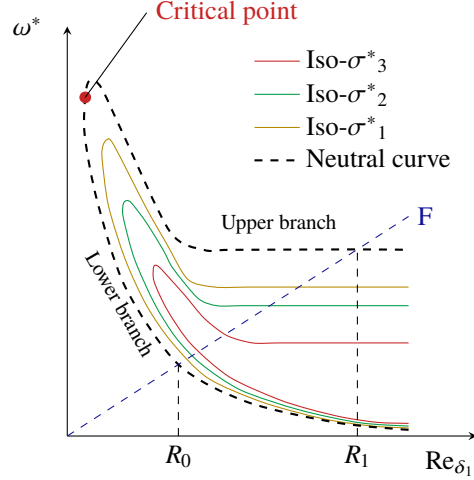
Fig. 2 Viscous-inflectional instabilities
