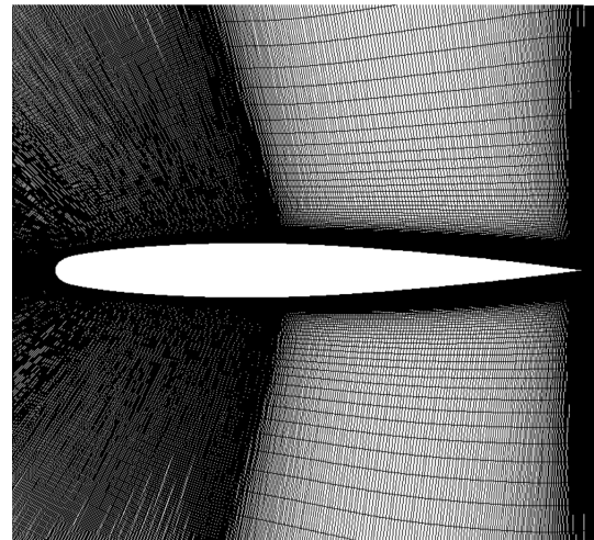
Fig. 12 Mesh around ONERAD airfoil
