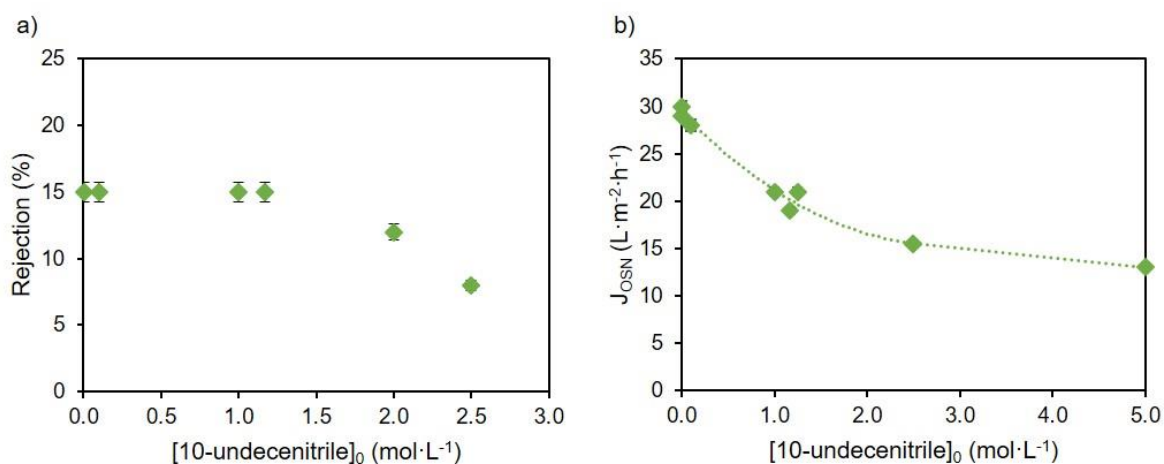
Figure 5. OSN of 10-undecitrile by Pervap 4060 in single toluene solution at 10 bar from 1 mM to 2.5 M. (a) Rejection up to VRR = 2; (b) Permeate flux in toluene, except 5 M corresponding to bulk (pure liquid) 10-undecitrile.
