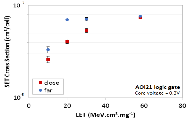
Fig. 2. SET cross section of AOI21 gate with transistor reordering technique under different LETs
