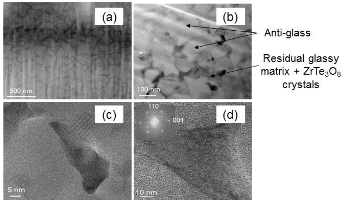
Figure 6: (a) and (b) STEM-HAADF images of glass-ceramic (2h, 340°C), (c) and (d) HRTEM and SAED (inset) patterns of ZrTe_3O_8 crystals
