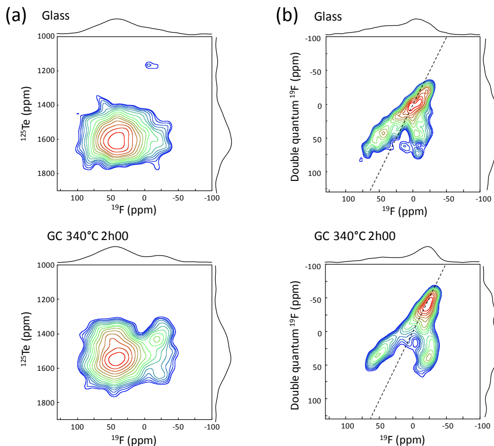
Figure 9: (a) ^{19}\text{F}\{-^{125}\text{Te}\} 2D HSQC MAS (60 kHz) spectra and (b) 2D ^{19}\text{F} homonuclear dipolar double-quantum correlation MAS (50kHz) spectra of the glass (top) and the glass-ceramic heat-treated at 340 °C for 2h (bottom).
