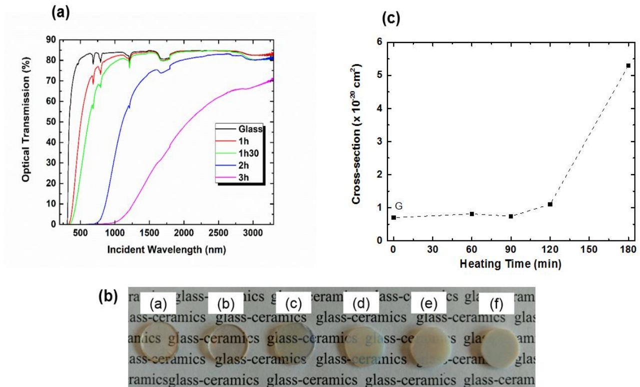
Figure 10: (a) Optical transmission data collected for the 1 at.% Tm^{3+} -doped 65TeO_2-35ZrF_4 samples (thickness \sim 1 mm) and displayed in the full range (200 – 3300 nm). (b) Photographs of the undoped 65TeO_2-35ZrF_4 composition: parent glass (a), glass-ceramics heat-treated at 340^\circ C for 30 min (b), 1h (c), 1h30 (d), 2h (e) and 3h (f). (c) Evolution of the absorption cross-section at \lambda = 792 nm (transition ^3H_6 - ^3H_4 ), for the 1 at.% Tm^{3+} -doped 65TeO_2-35ZrF_4 samples. Note that the G label stands for the glass sample.
