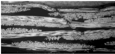
Figure 7. Contact compression till the rupture ( \approx 51 kN).
