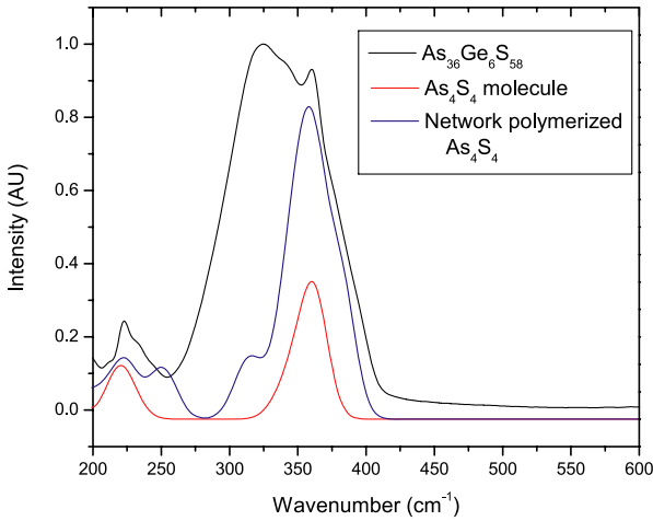
Fig. 9. Simulated Raman spectra of \text{As}_4\text{S}_4 molecule and polymerized network product, modeled using density functional theory.
