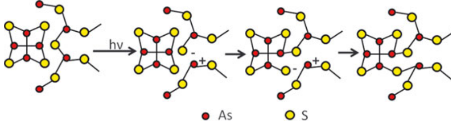
Fig. 8. Proposed mechanism for polymerization of \text{As}_4\text{S}_4 cluster into the glass network during irradiation.
