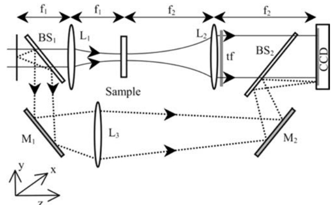
Figure 1. Experimental Z-scan setup. The labels refer to lenses ( L_1 and L_2 ), mirrors ( M_1 and M_2 ), beam splitters ( BS_1 and BS_2 ), and neutral filters (tf). The sample is moved in the focal region between L_1 and L_2 .
