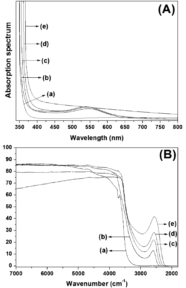
Figure 5. Linear absorption spectra (A) and infrared transmittance spectra (B) of the glass samples (a) FWB0, (b) FWB5, (c) FWB10, (d) FWB15, and (e) FWB20.
