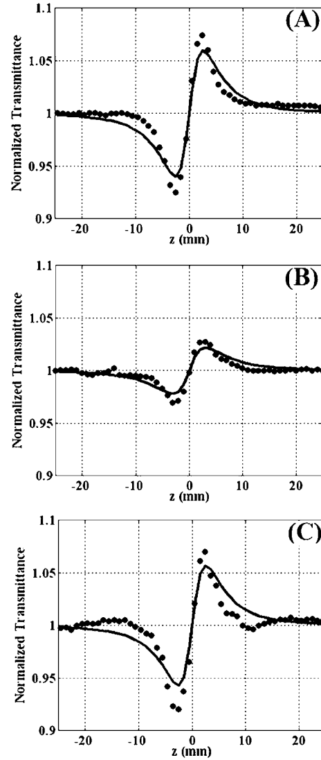
Figure 7. Closed-aperture Z-scan transmittances at 1064 nm. Experimental results (points) and theoretical fits (solid lines) for samples: (A) FWB5 (thickness of 1.23 mm and I_0 = 36 \text{GW}/\text{cm}^2 ); (B) FWB15 (thickness: 1.72 mm; I_0 = 20 \text{W}/\text{cm}^2 ); (C) FWB10 (thickness: 2.30 mm; I_0 = 4.5 \text{GW}/\text{cm}^2 ). I_0 is the on-axis peak intensity at the focus of lens L_1 of Figure 1.
