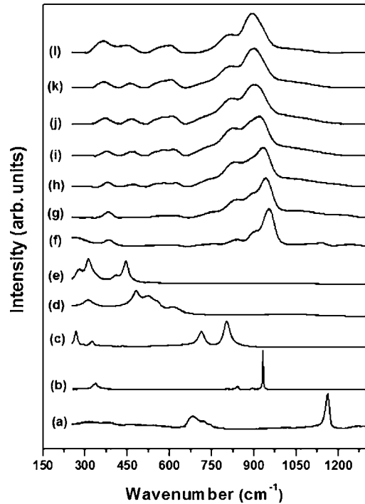
Figure 4. Raman spectra of the glass samples in the ternary system \text{NaPO}_3\text{-WO}_3\text{-Bi}_2\text{O}_3 and reference compounds: (a) \text{NaPO}_3 , (b) \text{NaWO}_4 , (c) \text{WO}_3 , (d) \text{NaBiO}_3 , (e) \text{Bi}_2\text{O}_3 , (f) FWB0, (g) FWB5, (h) FWB10, (i) FWB15, (j) FWB20, (k) FWB25, and (l) FWB30.
