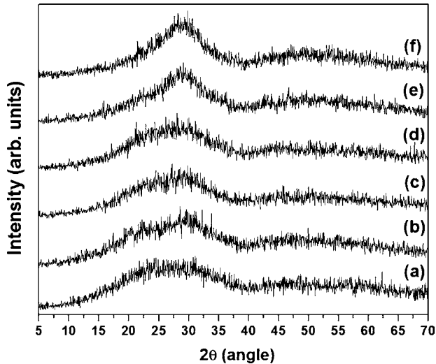
Figure 3. X-ray diffraction of the FWB glass samples (a) FWB5, (b) FWB10, (c) FWB15, (d) FWB20, (e) FWB25, and (f) FWB30.
