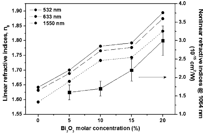
Figure 6. Linear refractive index (sphere-lines) and NL refractive index (square-line) behavior as a function of \text{Bi}_2\text{O}_3 molar concentration.
