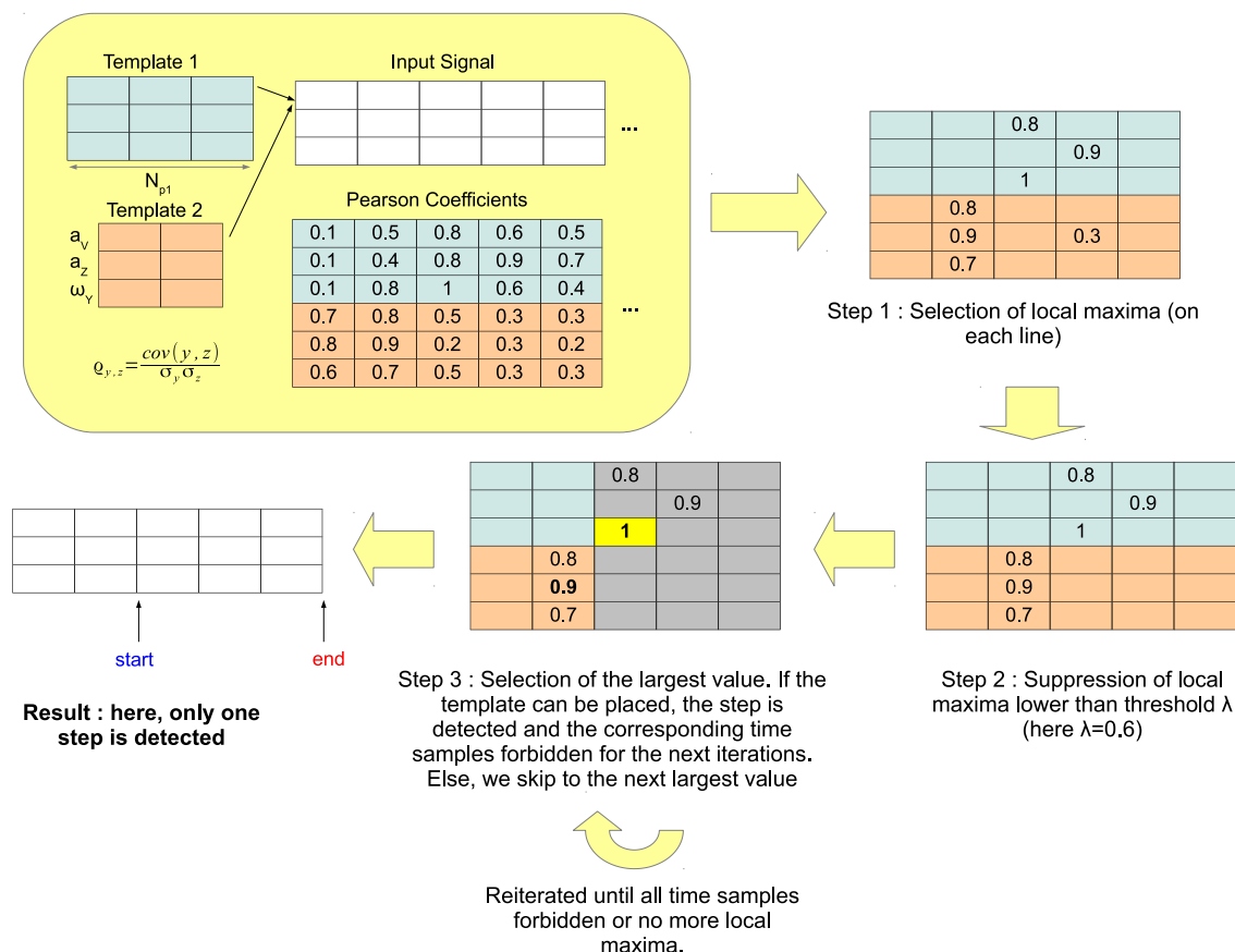
Figure 3. Chartflow of the step detection method.
