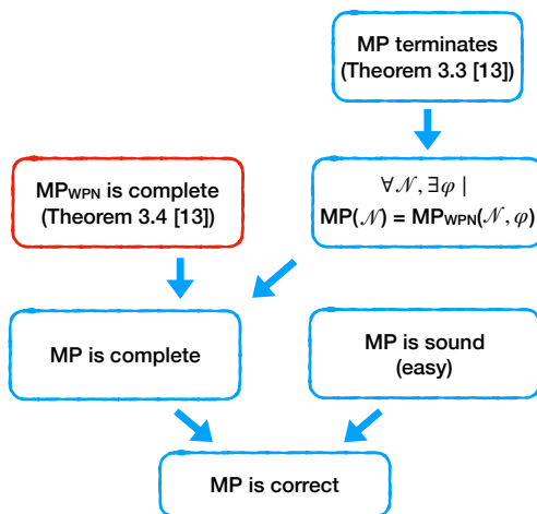
Fig. 3. Structure of the proof of [17]. The main difficulty lies in the completeness of \text{MP}_{\text{WPN}} , depicted in red.
