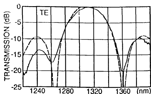
Fig. 6. Filter response for TE polarization ( \lambda g = 1.17 \mu\text{m} , rib height of 200 Å and 500 Å, 14 periods of 260 \mu\text{m} ), and calculations in dotted lines.
