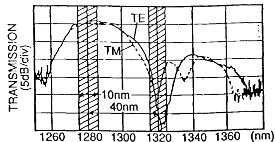
Fig. 5. Filter responses for both polarizations. The grating period is 132 \mu\text{m} and the coupling length equal to 16 grating periods.
