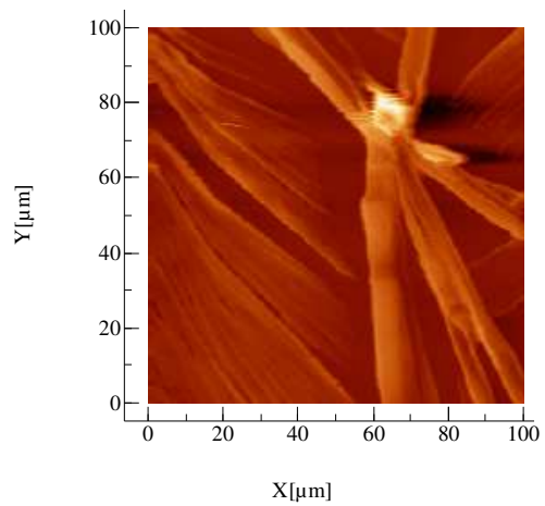
Figure-4. 2D and 3D AFM images for \text{CH}_3\text{NH}_3\text{PbI}_3 thin films deposited with different spin speeds on glass substrates.
