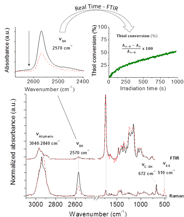
Figure 1. At the bottom, FTIR and Raman spectra of 3P film (solid line) and poly3P (dashed line) after 15 min UV irradiation with non-filtered Hg-Xe medium pressure mercury vapor lamp ( 490 \text{ mW.cm}^2 ). At the top, the enlarged section shows the evolution of thiol IR stretching mode at 2570 \text{ cm}^{-1} (left); rapid scan analysis was exploited to obtain thiol conversion-time plot (right).
