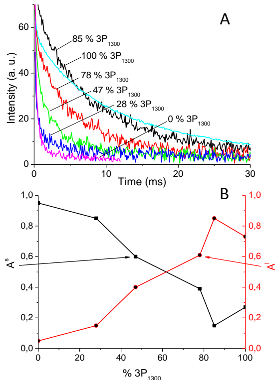
Figure 7. A. Decay of the transverse magnetization for polydisulfide copolymer network derived from 3P/3P_{1300} . B. Effect of 3P_{1300} weight concentration on fractional amplitude of the short ( A^s , T_2 < 0.5 ms) and long relaxation components ( A^l , T_2 > 0.5 ms).
