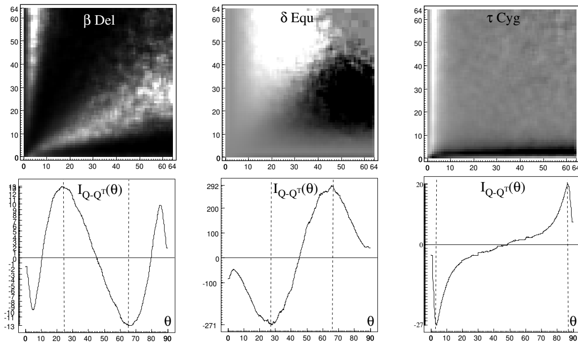
Fig. 3. Gray-level plots of function Q - Q^T , and plots of its radial integration I_{Q-Q^T} , computed on the specklegrams of three binary stars. The radial integrations show two extrema. The maximum is reached for \arctan(\alpha) , the minimum for \arctan(1/\alpha) , \alpha being the intensity ratio of the two binary components. A value of \alpha < 1 means that the spatial lag vector goes from the brightest star to the lowest. The opposite if \alpha > 1 . This gives the absolute position angle of the couple.
